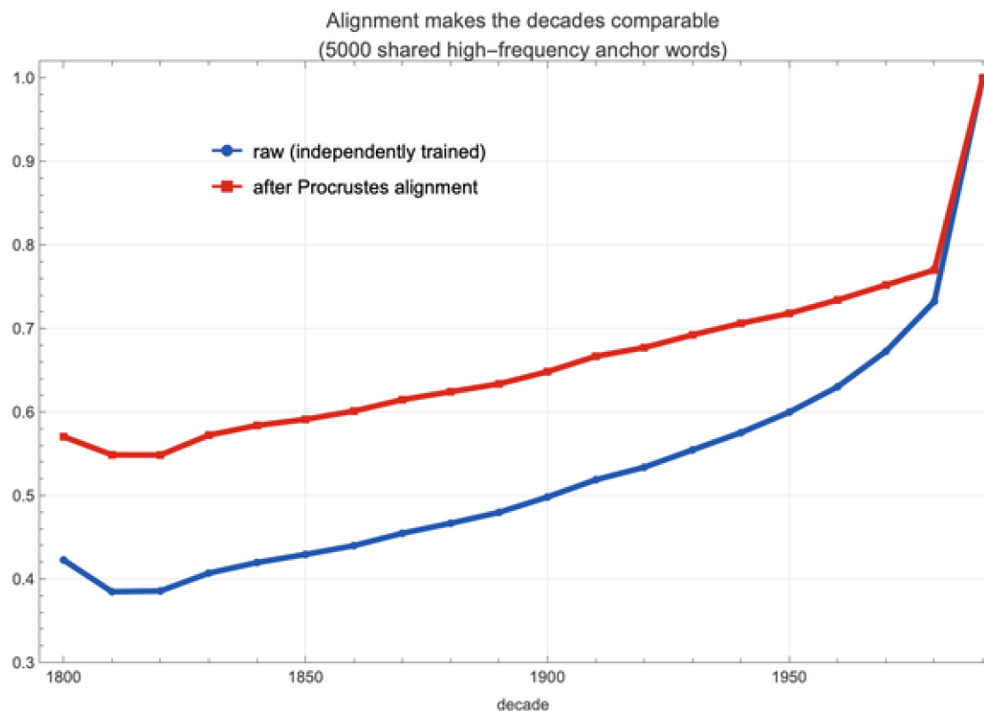
Figure. Mean cosine of the 5,000 shared anchor words to their 1990s vectors, before (blue) and after (red) Procrustes alignment. Alignment lifts the curve at every decade; both necessarily reach 1.0 at the 1990s reference.
