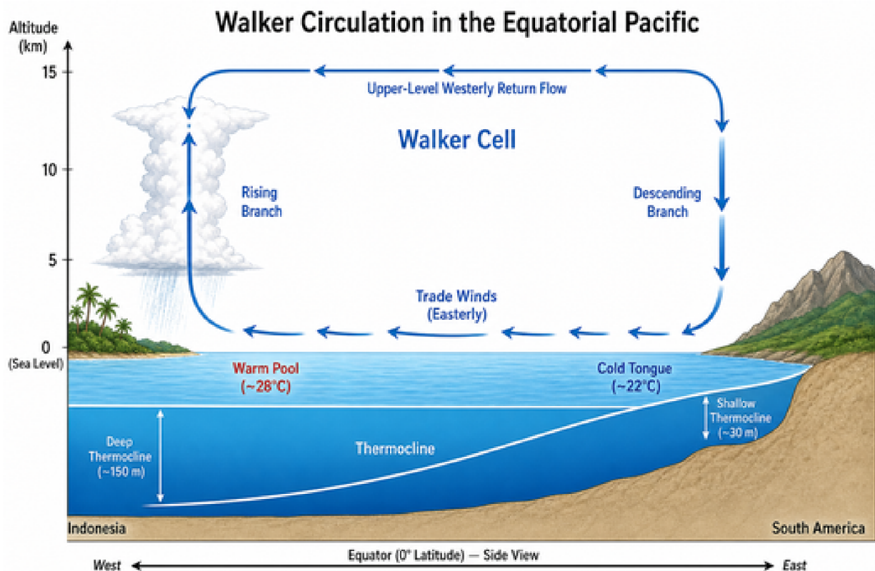
Figure 1.2 Schematic of the climatological Walker circulation along the equator. Easterly trade winds at the surface, rising air over the Indonesian warm pool, upper-level westerly return flow, descending air over the cool eastern Pacific. During El Niño the trades weaken, the thermocline flattens, and the rising branch shifts east toward the dateline. Generated with OpenAI gpt-image-2.
