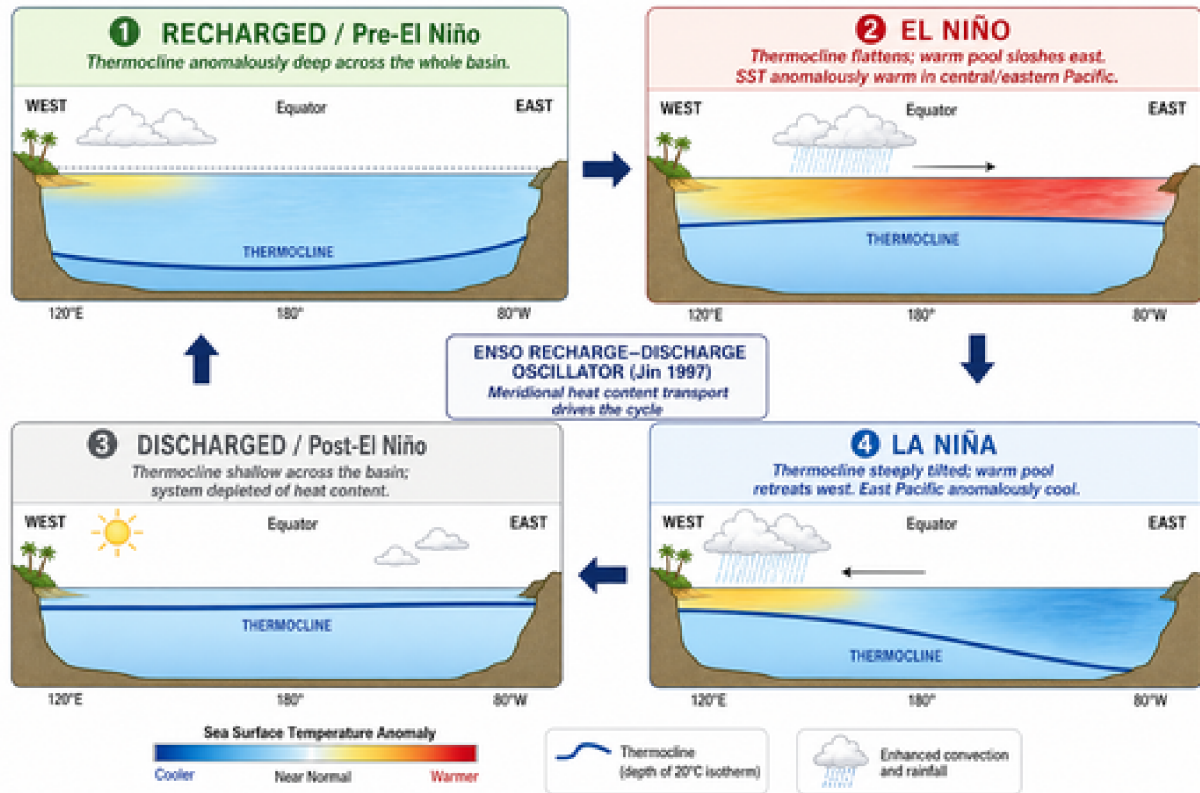
Figure 5.1 The four phases of the recharge-discharge ENSO cycle (Jin 1997), drawn schematically. (I) Pre-event recharge: thermocline anomalously deep across the basin, heat content elevated. (II) El Niño: warm pool sloshes east, thermocline flattens, eastern SST anomalously warm. (III) Discharge: basin-wide upper-ocean heat content depleted by poleward Sverdrup transport during the event. (IV) La Niña: thermocline steeply tilted, eastern cold tongue intensified. The cycle then restarts. Generated with OpenAI gpt-image-2.
