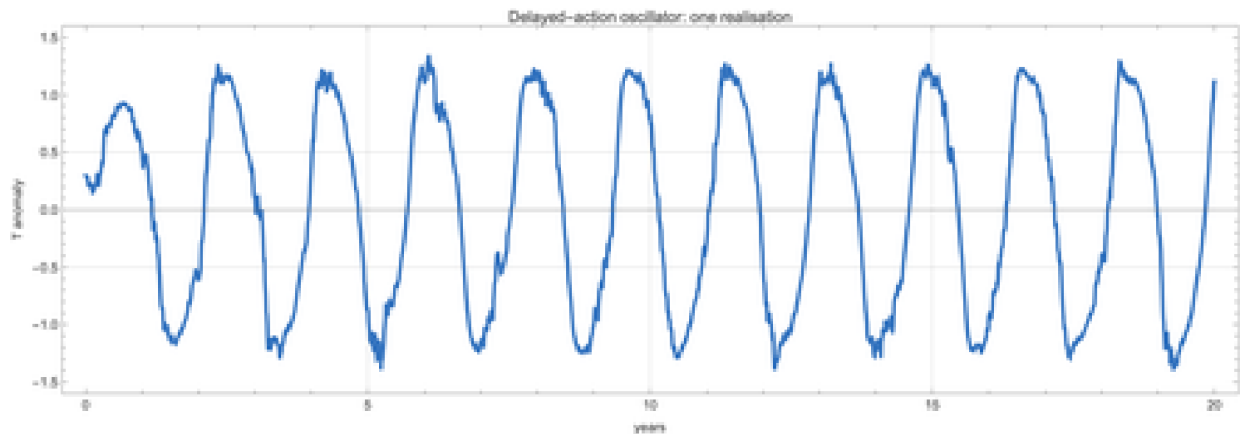
Figure 5.8 A 20-year realisation of the delayed oscillator with \alpha = 0.75 (well above the Hopf threshold) and \delta = 6 months. The limit cycle period is approximately 4\delta = 24 months — shorter than the canonical ENSO period — but the nonlinear-oscillator phenomenology is correct.
