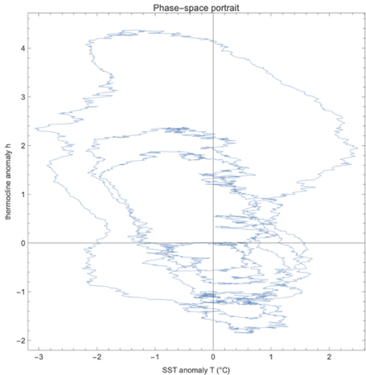
Figure 5.3 Single 20-year stochastic realisation of the recharge-discharge oscillator with seasonally modulated coefficients. Period is irregular (3–6 years) and amplitude is variable, as in observations.
