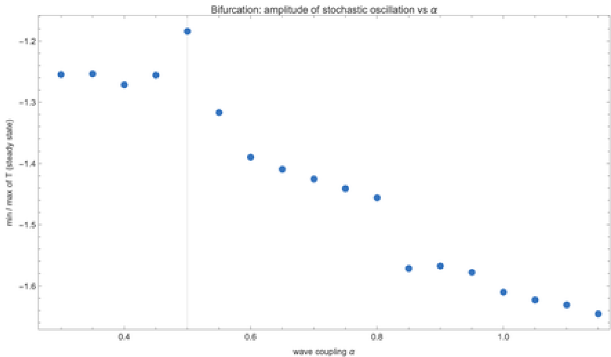
Figure 5.7 Min and max of T in long stochastic runs of the delayed oscillator, as a function of the wave-coupling \alpha , with \delta = 3 (= 6 months) held fixed. The Hopf bifurcation at \alpha \approx 0.5 is the transition from noise-driven fluctuations about the fixed point to a sustained nonlinear limit cycle.
