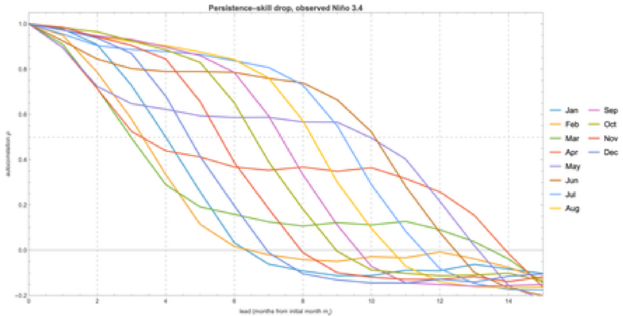
Figure 4.3 Persistence-skill curves: \rho vs lead for each starting calendar month. Lines that start in boreal winter and spring (Jan, Feb, Mar, Apr) drop steeply through the first six leads; lines that start in summer and autumn (Jul, Aug, Sep, Oct) retain \rho > 0.5 out to lead 9.
