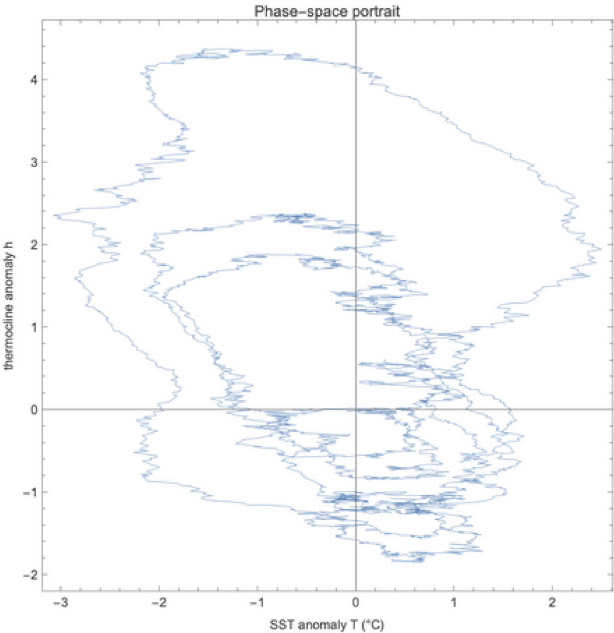
Figure 5.3 Single 20-year stochastic realisation of the recharge-discharge oscillator with seasonally modulated coefficients. Period is irregular (3–6 years) and amplitude is variable, as in observations.
