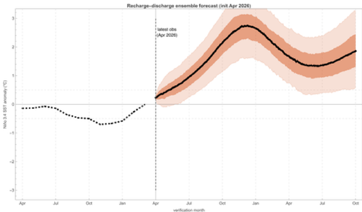
Figure 6.1 Recharge–discharge oscillator live ensemble forecast initialised from observed April 2026 state ( T = +0.23\text{ }^\circ\text{C} , inferred h \approx +4.9 ). Dotted line shows the past 12 months of observations. The solid black line is the ensemble median; the darker orange band is the 25–75 % inter-quartile range; the lighter orange band is the 5–95 % confidence interval. The model peaks the event at +2.0 to +3.0 °C around DJF 2026–27, broadly consistent with the NOAA 96 % El-Niño probability for that season.
