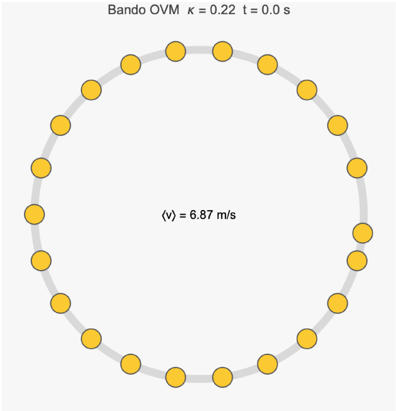
Figure 9. Animated Bando OVM. The ring starts in near-uniform flow; a small perturbation rotates around the ring, grows, and breaks the symmetry into a persistent stop-and-go wave.
