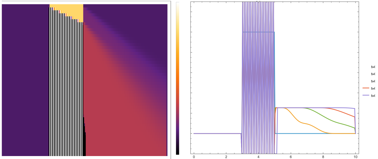
Figure 2. LWR density evolution on a 10 km corridor with an initial density block. Left: space-time heatmap; the bright diagonal streak is the backward-propagating shock. Right: snapshots at five increasing times showing the jam block dissolve into a backward shock (left edge) and a forward rarefaction (right edge).
