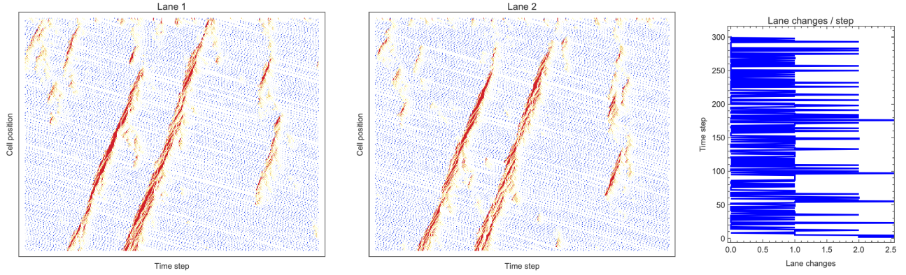
Figure 12. Two-lane NaSch with 150 vehicles (75 per lane initially). Left two panels: per-lane space-time diagrams. Right: number of lane changes per step. Peaks in lane-change activity coincide with density imbalances between the two lanes.
