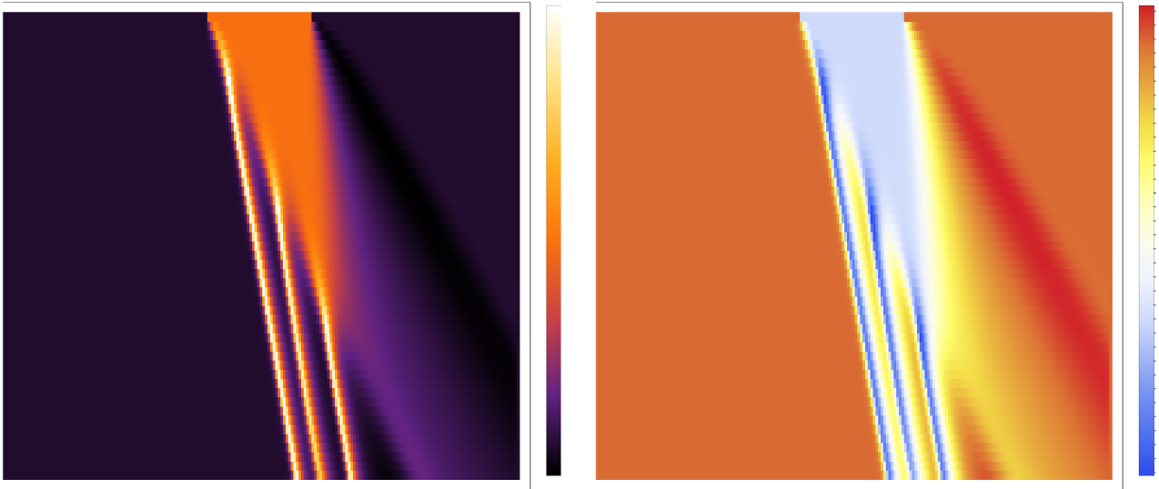
Figure 4. Payne–Whitham density (left) and velocity (right) evolution near a merge zone. Unlike LWR the velocity can drop below equilibrium transiently, producing stop-and-go oscillations rather than a clean shock.
