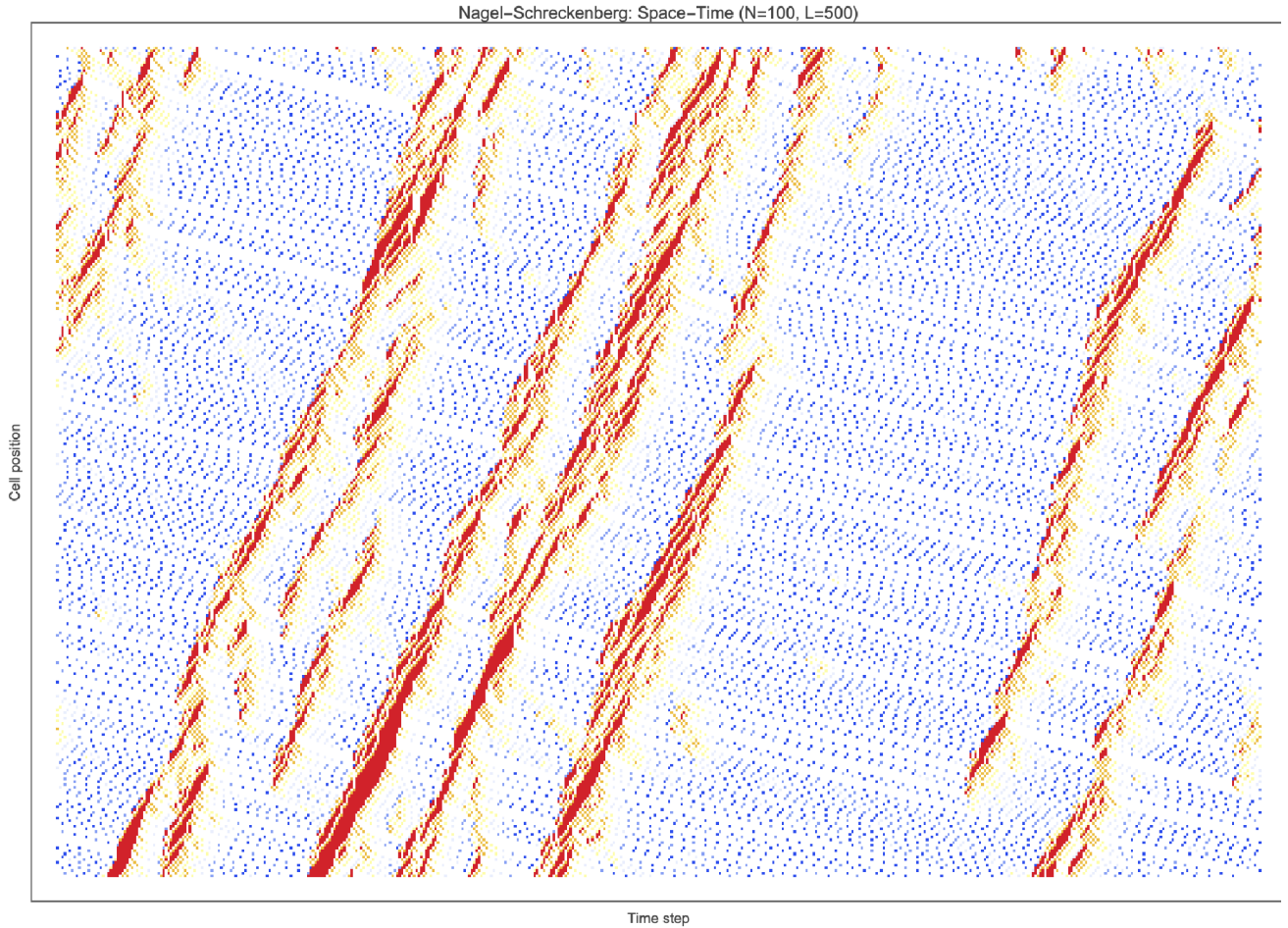
Figure 10. Space-time diagram of 100 NaSch vehicles on a 500-cell periodic lattice over 300 steps, with randomisation probability p=0.3 and v_{\text{Max}}=5 cells/step. The diagonal dark bands are jam waves moving upstream (leftward) relative to the vehicles, which move rightward.
