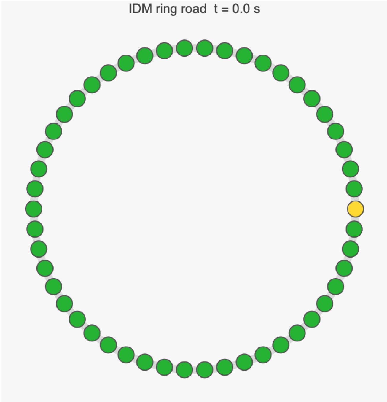
Figure 7. The same ring road animated. One vehicle started at half speed; the instability propagates around the ring and crystallises into a persistent stop-and-go wave.
