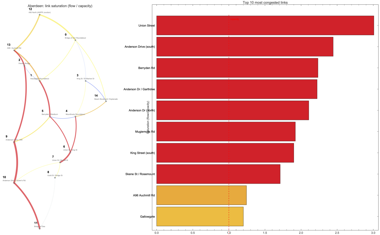
Figure 17. Equilibrium on the realistic 15-node Aberdeen network. Left: saturation map of the 23 roads; the thickest red edge is Union Street. Right: top ten most-congested links, with Union Street at 3.0x capacity followed by Anderson Drive (south) and Berryden Road.
