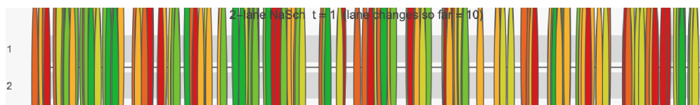
Figure 7. Two-lane NaSch with 150 vehicles (75 per lane initially). The running counter in the title shows cumulative lane-change events; each occurs when a vehicle would otherwise have to brake but the other lane satisfies the gap-acceptance criteria. (MP4: Wolfram/results/anim_nasch_2lane.mp4 .)
