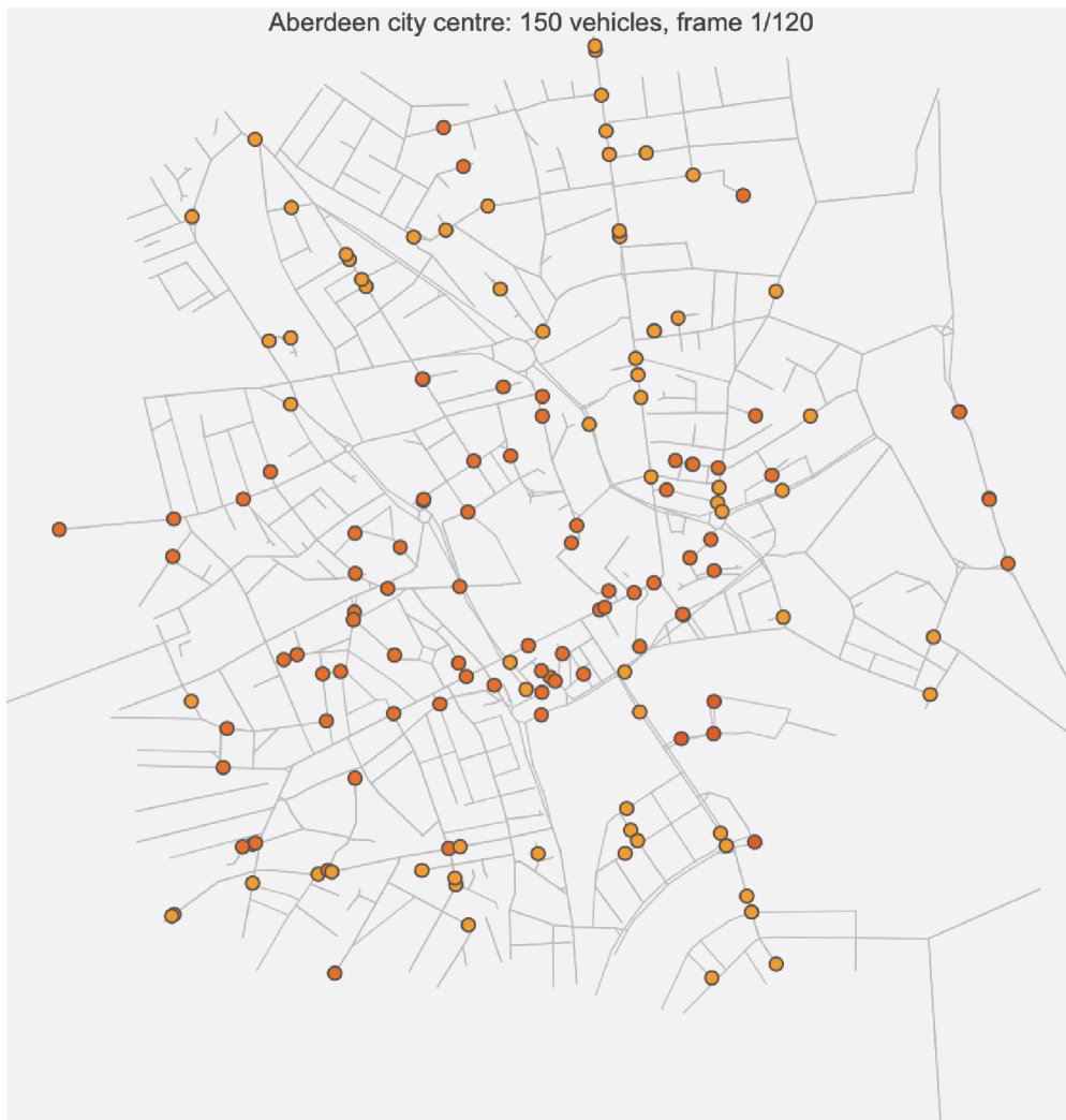
Figure 16. Zoomed-in view: 150 vehicles on the 800 m radius city-centre extract (1397 drivable nodes). Union Street cuts diagonally through the middle; Marischal College is at the centre. At this scale individual vehicle interactions and queue build-up at intersections are very visible. (MP4: Wolfram/results/aberdeen_city.mp4 .)
