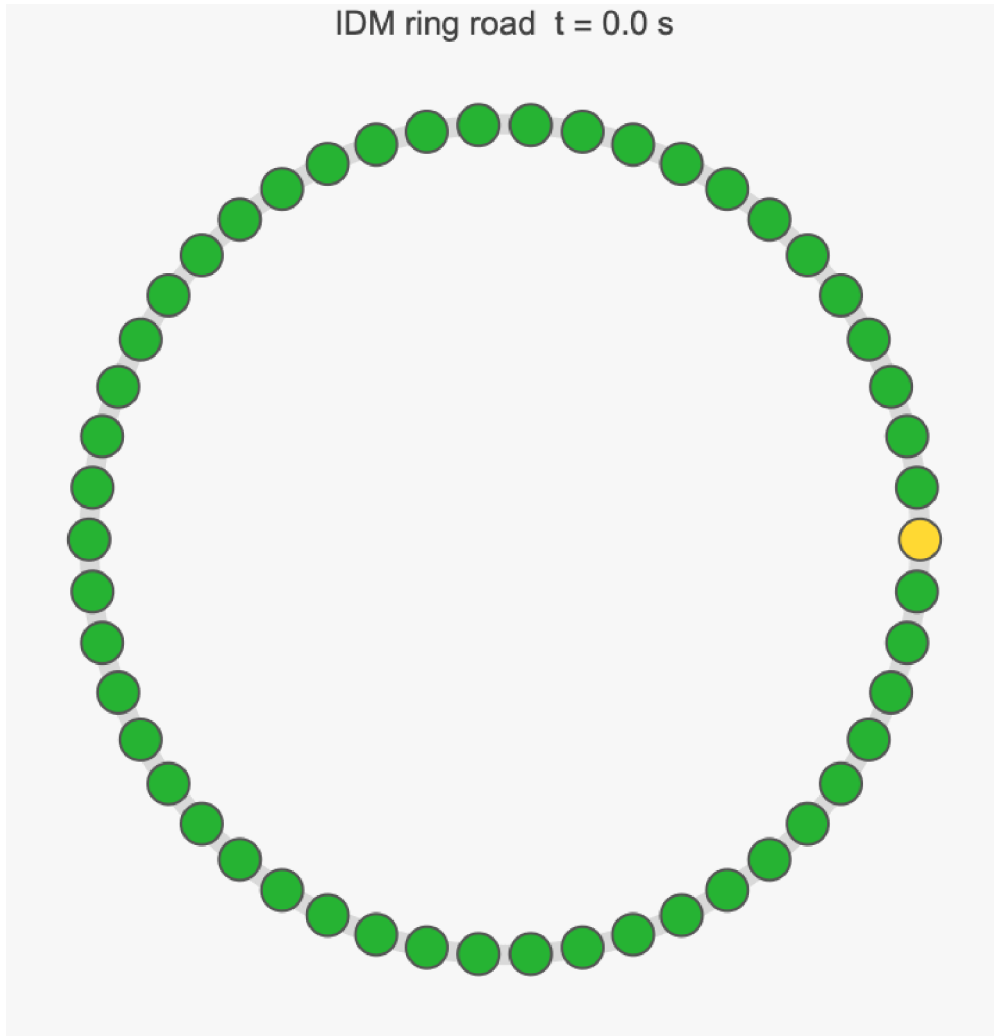
Figure 4. 50 IDM vehicles on a 1 km ring road. One vehicle is seeded at half speed at t=0 ; the instability propagates backward around the ring and crystallises into a persistent stop-and-go wave. Each disk is a vehicle coloured by its instantaneous speed (green = free flow, red = stopped). (MP4: Wolfram/results/anim_idm.mp4.)
