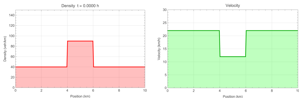
Figure 3. Animated Payne-Whitham run near a merge zone. Unlike LWR the velocity field can drop below equilibrium transiently, producing stop-and-go oscillations rather than a clean shock. (MP4: Wolfram/results/anim_payne_whitham.mp4 .)
