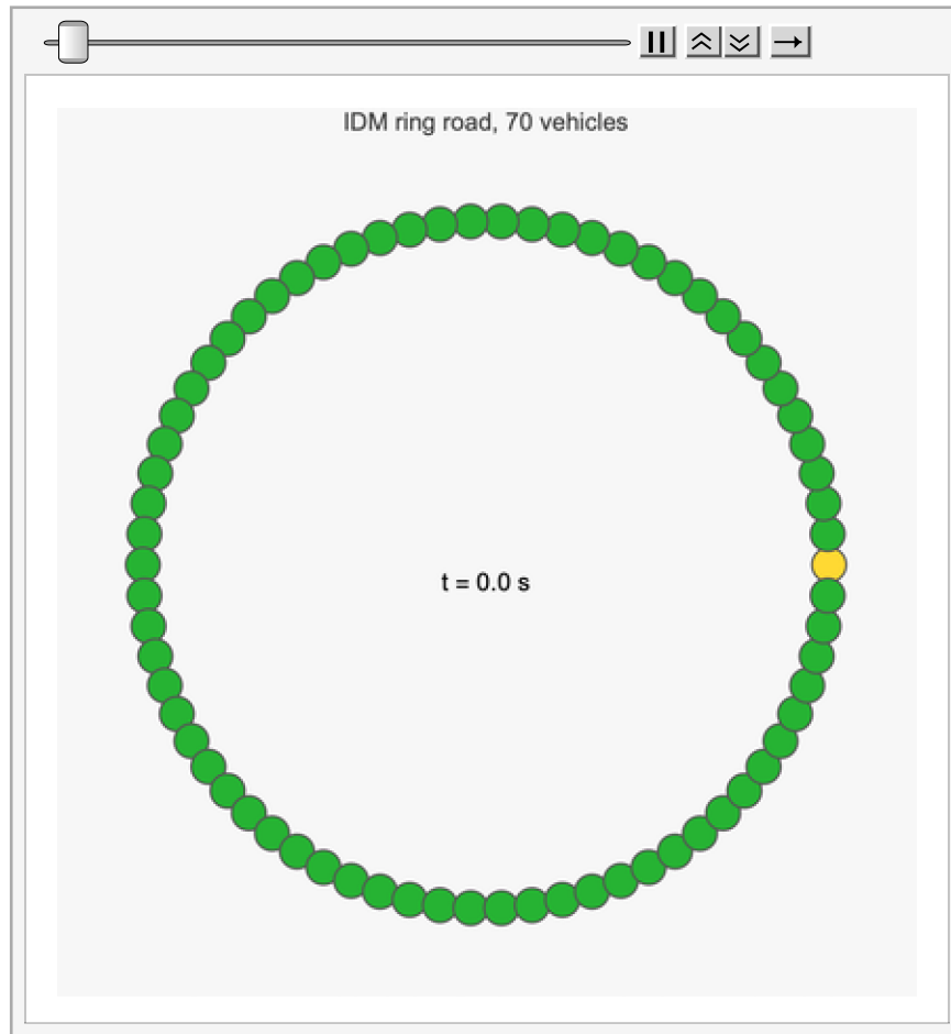
Figure 4. 70 IDM vehicles on a 2 km ring road with Treiber's phantom-jam parameters ( v_0=30 m/s, T=1.6 s, a=0.73 m/s 2 , b=1.67 m/s 2 ). One vehicle is seeded at half speed at t=0 ; after a few seconds the instability amplifies through the platoon into a persistent stop-and-go wave that rotates backward around the ring. By t=400 s speeds span 0.9 to 20.6 m/s -- the dense red cluster is the jam, the green free-flow arc is downstream of it. (MP4: Wolfram/results/anim_idm.mp4 .)
