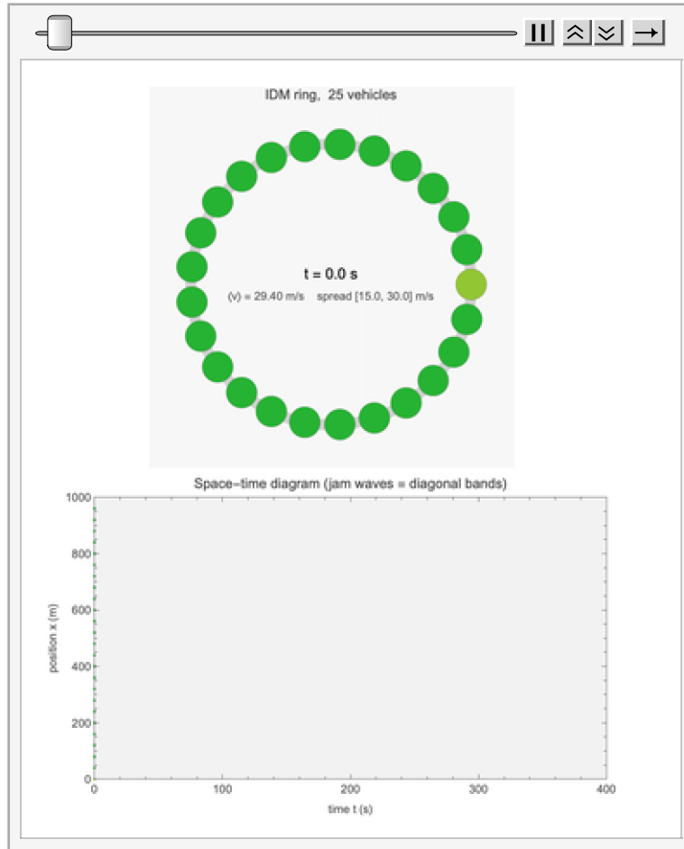
Figure 4. 25 IDM vehicles on a 1 km ring with an extreme phantom-jam configuration ( v_0=30 m/s, T=2.5 s, a=0.3 m/s 2 , b=2.0 m/s 2 ). At t=0 the cars are visibly spaced out (40 m mean gap) at free-flow speed. A single-vehicle speed perturbation amplifies; by t=400 s the ring has a deep-red cluster of near-stopped cars (slowest \sim 0.8 m/s) next to a green free-flow arc (fastest \sim 17 m/s). Bottom panel: accumulating space-time trajectory diagram (time along x, position along y with wrap-around at 1000 m). The backward-travelling jam wave is the diagonal red band – cars move forward (slope up-right) but the jam drifts backward relative to them. (MP4: Wolfram/results/anim_idm.mp4 .)
