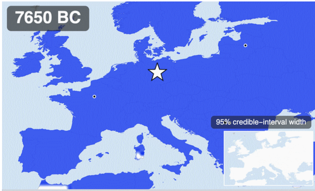
Forward simulation from the fitted point source: posterior mean over 100 origin–model draws, 100–year interpolated steps from 9,600 BP. Generated by ExportOriginSpread ; the H.264 version is figures/generated/origin_spread.mp4 .
