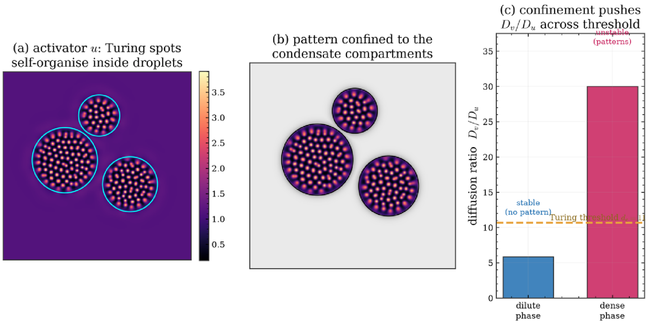
Figure 10.9 Intra-droplet Turing patterns. The activator field forms spots inside the condensates and stays flat in the dilute phase (42 \times amplitude contrast); the bar chart shows D_v/D_u crossing the Schnakenberg threshold d_c = 10.7 inside.
