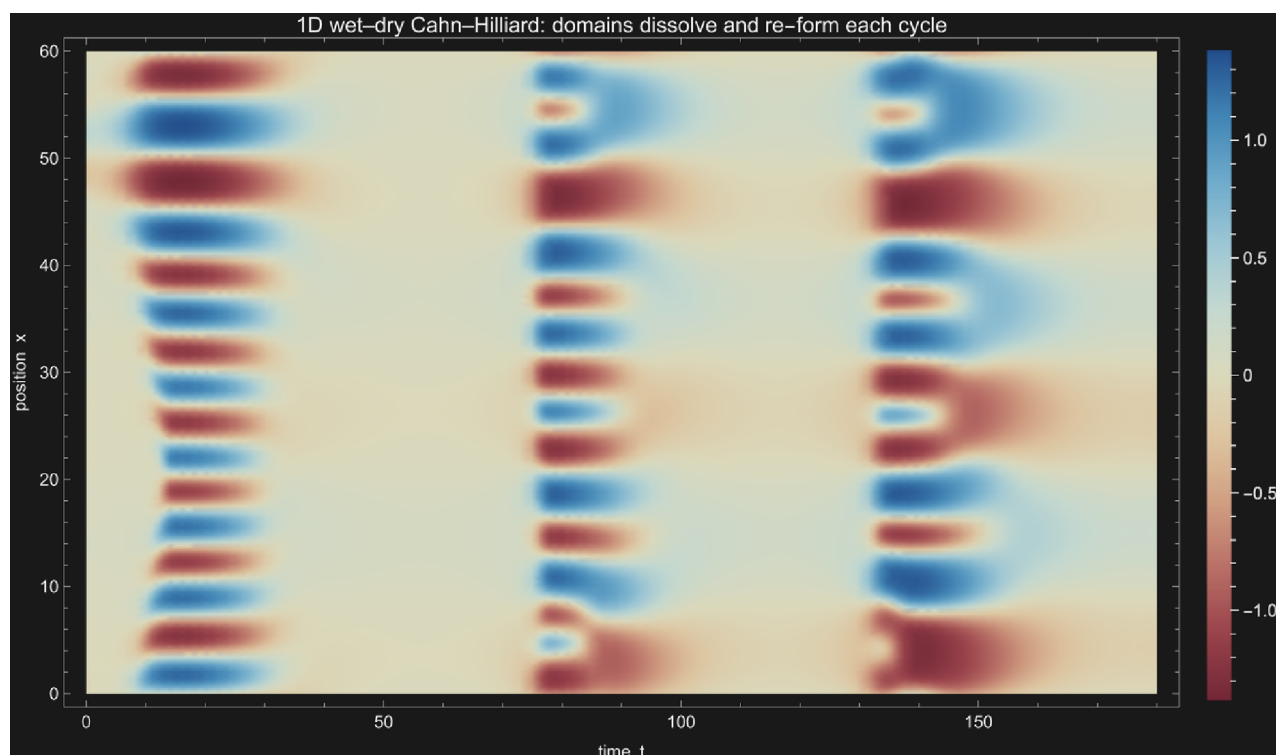
Figure 10.13 (Wolfram NDSolve.) 1D wet-dry Cahn-Hilliard space-time: domains dissolve at each wet half-cycle and re-form at each dry half-cycle.
