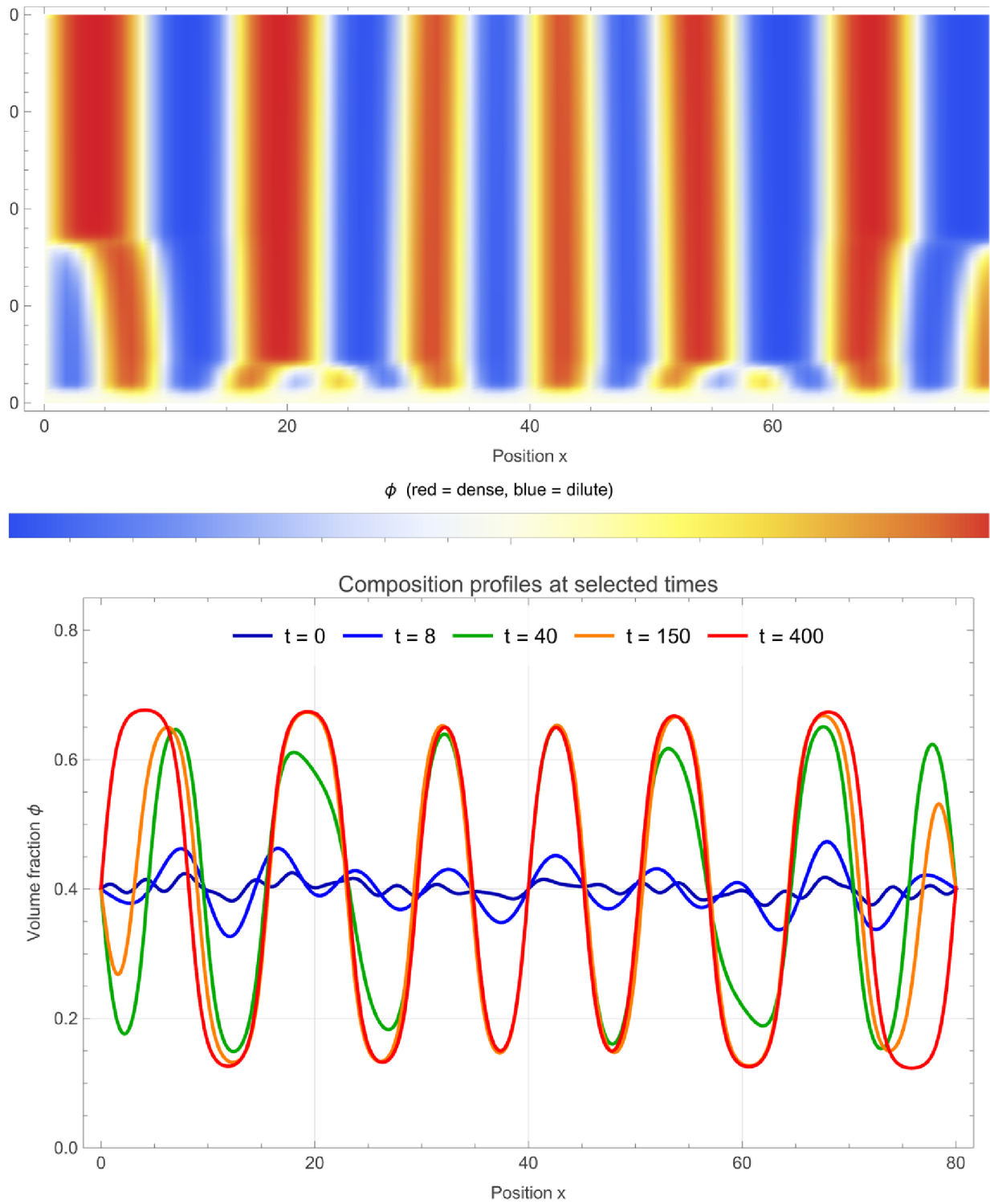
Figure 3.1 Top: space-time density plot of the 1D spinodal decomposition. The initially uniform composition rapidly develops concentration fluctuations that coarsen into well-separated dense (red) and dilute (blue) domains. Bottom: composition profiles at selected times showing the progression from small perturbation to fully phase-separated condensates.
