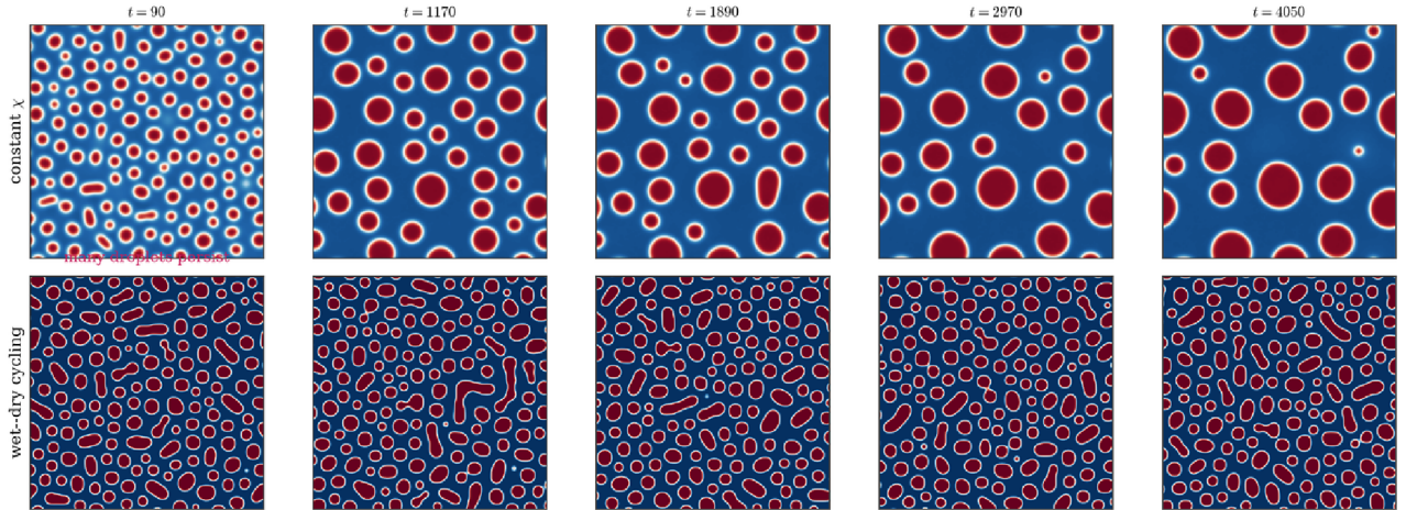
Figure 10.12 The same contest seen in the 2D droplet fields. Top row (constant \chi ): Ostwald ripening coarsens the emulsion toward a few large winners. Bottom row (wet-dry cycling): each dissolution half-cycle wipes out the size differences that drive ripening, so a dense population of comparable droplets is continually regenerated.
