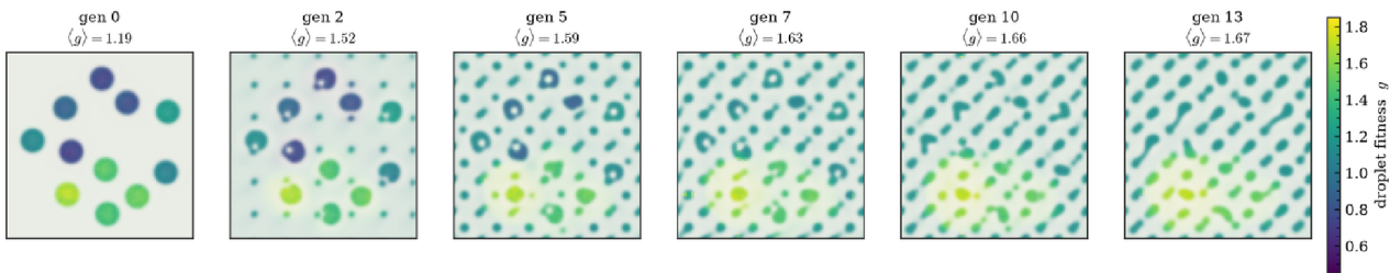
Figure 10.5 Snapshots of the droplet field coloured by fitness (yellow = fitter). Low-fitness (blue) droplets dissolve while fit droplets proliferate by fission and dominate the population.
