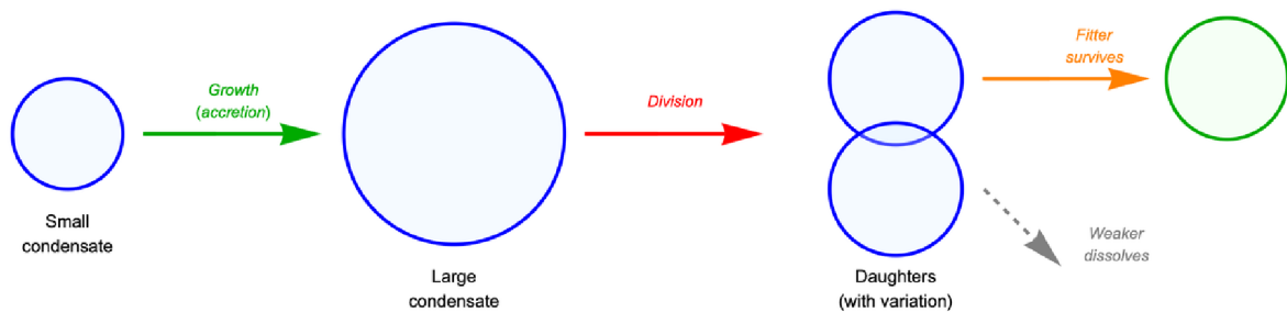
Figure 6.1 Schematic of the protocell life cycle. Small condensates grow by accretion of material from the bulk and by internal replication. When they exceed a critical size, mechanical instability drives division into two daughters. Daughters inherit (with variation) the parent's composition, including its partition coefficient K and replication efficiency. Weaker daughters dissolve; fitter ones survive and grow.
