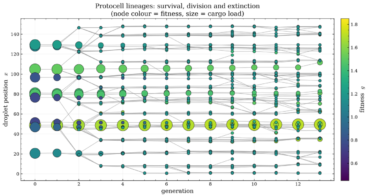
Figure 10.6 Protocell lineages: a genuine phylogeny in which the fit (yellow) lineage branches and takes over while low-fitness lineages go extinct (node colour = fitness, size = cargo load).
