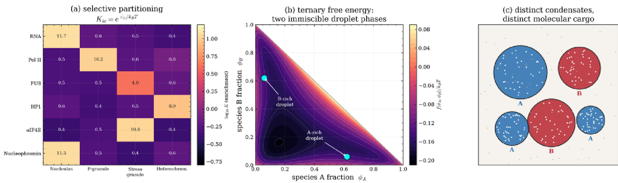
Selective compartmentalization: different species partition into different condensates
