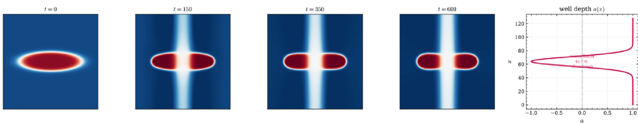
Figure 9.5 (Python 2D spectral solver.) An elongated droplet (left) is divided by a central warm band where the well depth a(x) dips below zero (right): the neck dissolves and two daughter droplets pinch off, conserving mass.
