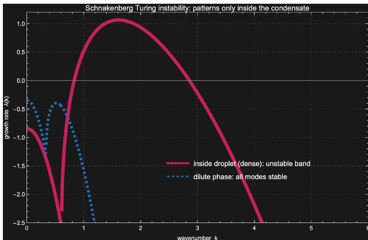
Figure 10.10 (Wolfram.) Schnakenberg linear-stability growth rate: a band of wavenumbers is unstable inside the dense phase while every mode is stable in the dilute phase.
