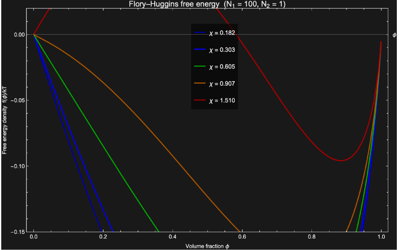
Figure 2.1 Flory-Huggins free energy density for a polymer-solvent system ( N_1 = 100 , N_2 = 1 ) at several values of \chi . Below the critical \chi , the free energy has a single minimum (stable mixed state). Above it, a double well appears: the system phase-separates into dilute ( \phi_L ) and dense ( \phi_D ) phases at the two minima.
