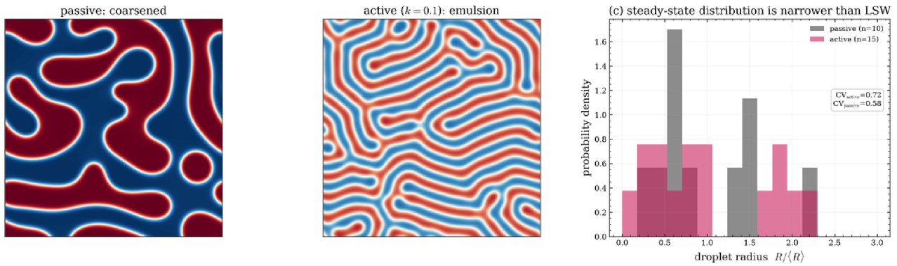
Steady-state emulsion vs. passive coarsening: morphology and size distribution
