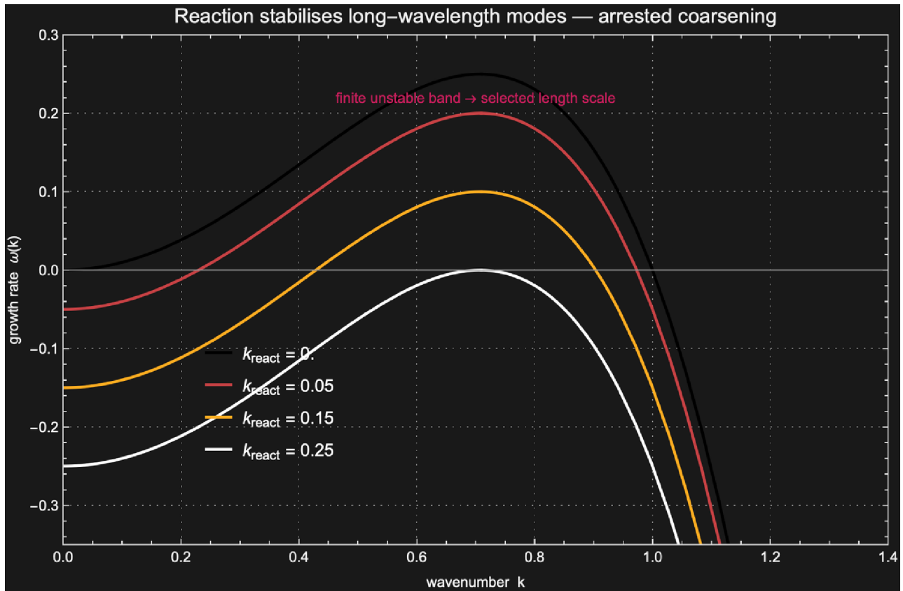
Figure 9.1 Reaction-modified dispersion relation. Increasing the reaction rate pushes the small- k (long-wavelength) modes below zero, leaving a finite unstable band -- coarsening can no longer proceed to arbitrarily large domains.
