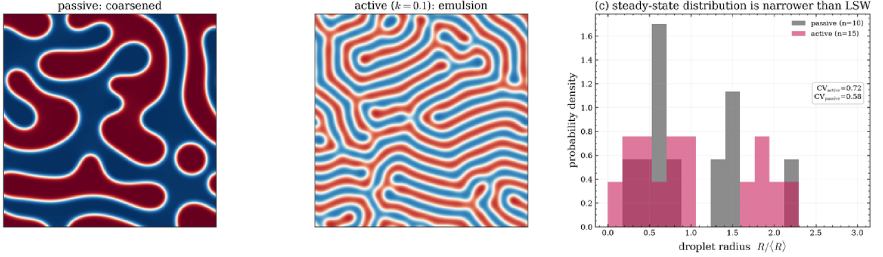
Steady-state emulsion vs. passive coarsening: morphology and size distribution
