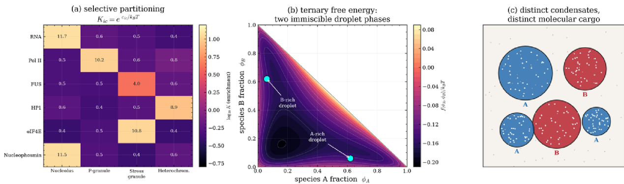
Figure 10.2 Selective compartmentalization. (a) Boltzmann partition coefficients send each client to its preferred condensate. (b) A ternary (A, B, solvent) free energy with two immiscible minima. (c) Distinct droplets carry distinct molecular cargo.
