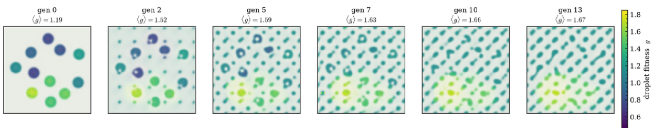
Figure 10.5 Snapshots of the droplet field coloured by fitness (yellow = fitter). Low-fitness (blue) droplets dissolve while fit droplets proliferate by fission and dominate the population.
