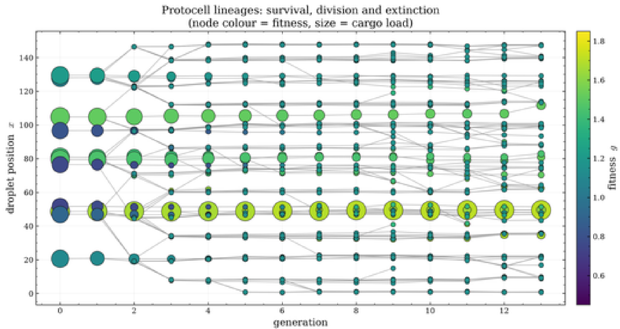
Figure 10.5 Protocell lineages: a genuine phylogeny in which the fit (yellow) lineage branches and takes over while low-fitness lineages go extinct (node colour = fitness, size = cargo load).
