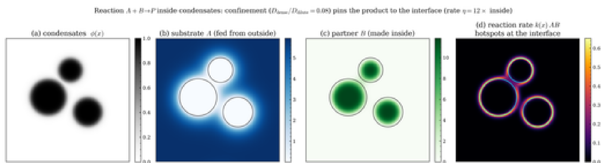
Figure 10.7 A+B \rightarrow P inside condensates. Confinement ( D_{\text{dense}}/D_{\text{dilute}}=0.08 ) keeps substrate A in an outer shell where it meets the interior partner B ; the product (rightmost panel) forms in a ring at the interface.
