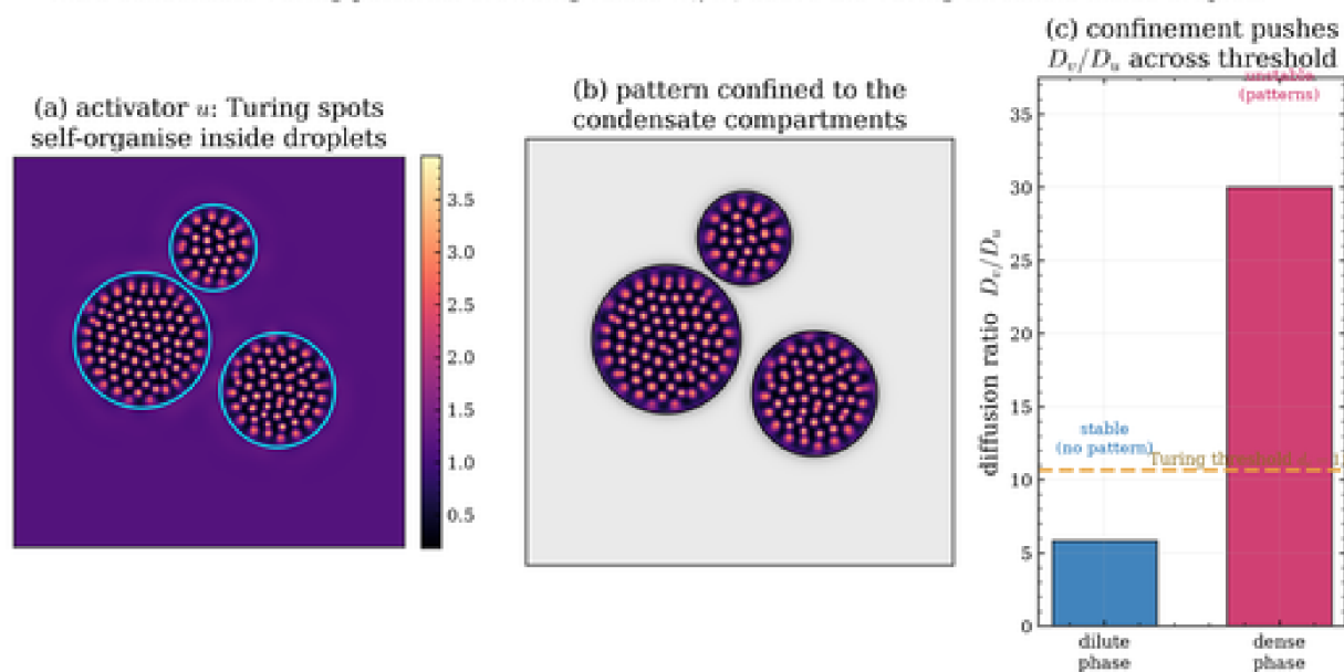
Figure 10.8 Intra-droplet Turing patterns. The activator field forms spots inside the condensates and stays flat in the dilute phase (42 \times amplitude contrast); the bar chart shows D_v/D_u crossing the Schnakenberg threshold d_c=10.7 inside.
