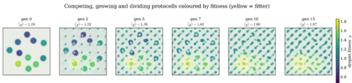
Figure 10.3 (a) Population mean fitness rises 1.19→1.67 over 14 generations and saturates below g_{\text{max}} . (b) The cargo-weighted genotype distribution shifts toward fitter replicators.
