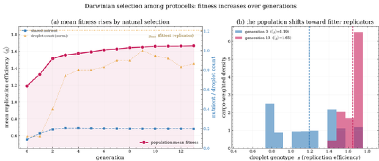
Figure 10.3 (a) Population mean fitness rises 1.19→1.67 over 14 generations and saturates below g_{\text{max}} . (b) The cargo-weighted genotype distribution shifts toward fitter replicators.
