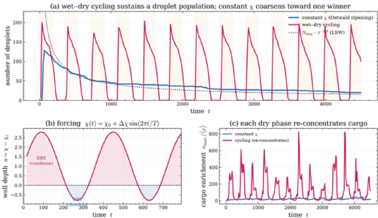
Figure 10.10 Droplet number over time: under wet-dry cycling the population is repeatedly reset and sustained, whereas constant \chi coarsens away as the Lifshitz-Slyozov t^{1/3} law. Each dry phase also re-concentrates cargo (a prebiotic ratchet).
