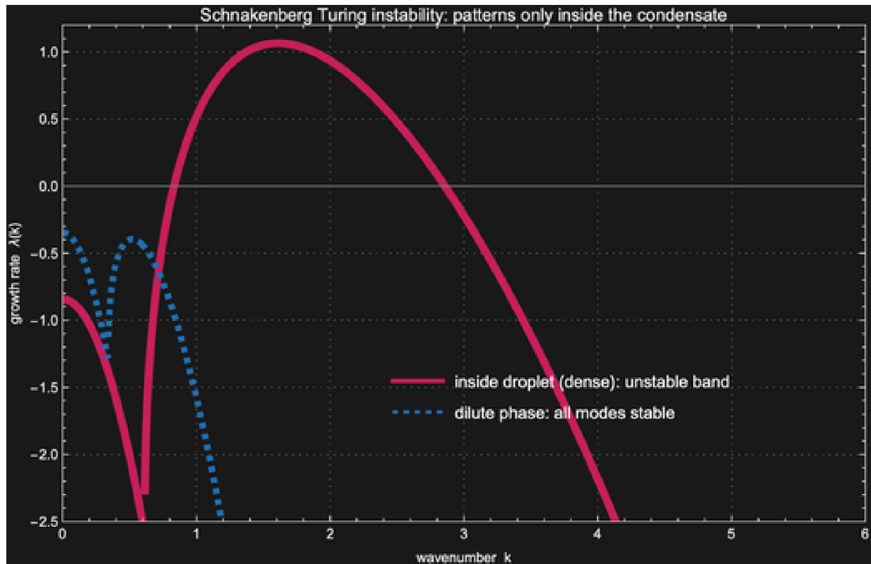
Figure 10.9 (Wolfram.) Schnakenberg linear-stability growth rate: a band of wavenumbers is unstable inside the dense phase while every mode is stable in the dilute phase.
