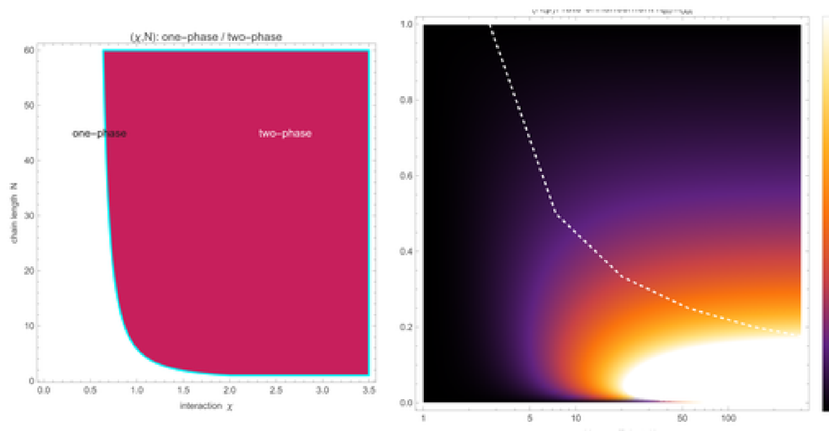
Figure 10.13 (Wolfram.) The two analytic planes rendered natively: the (\chi, N) two-phase region and the (K, p) rate-enhancement landscape with the p^* \approx 1/K ridge.
