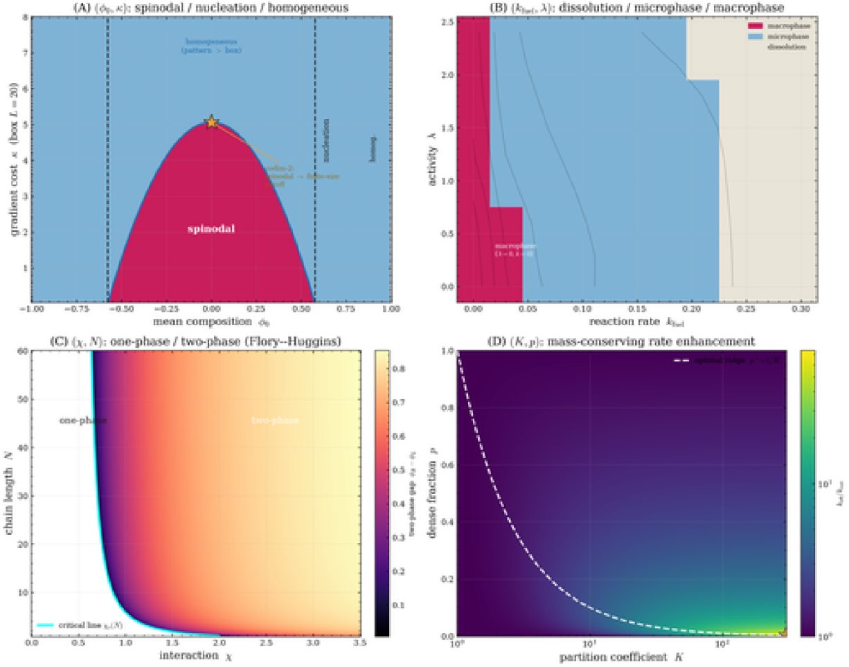
Figure 10.12 The condensate model's parameter space. (A) (\phi_0, \kappa) : spinodal / nucleation / homogeneous, with the codim-2 apex where the spinodal meets the finite-size cutoff. (B) (k_{fuel}, \lambda) : dissolution / microphase / macrophase from short 2D simulations. (C) (\chi, N) : Flory-Huggins two-phase region and critical line. (D) (K, p) : rate enhancement with the optimal ridge.
