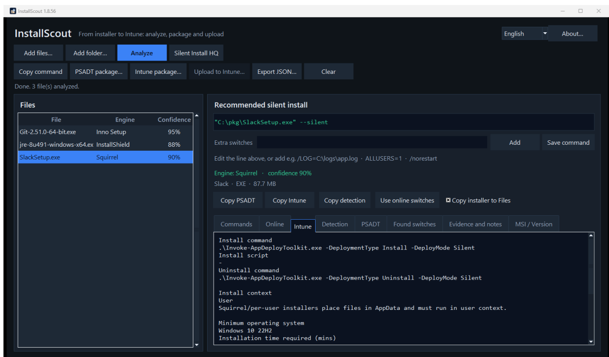
Figure 7. Squirrel/Slack with Install context User.
