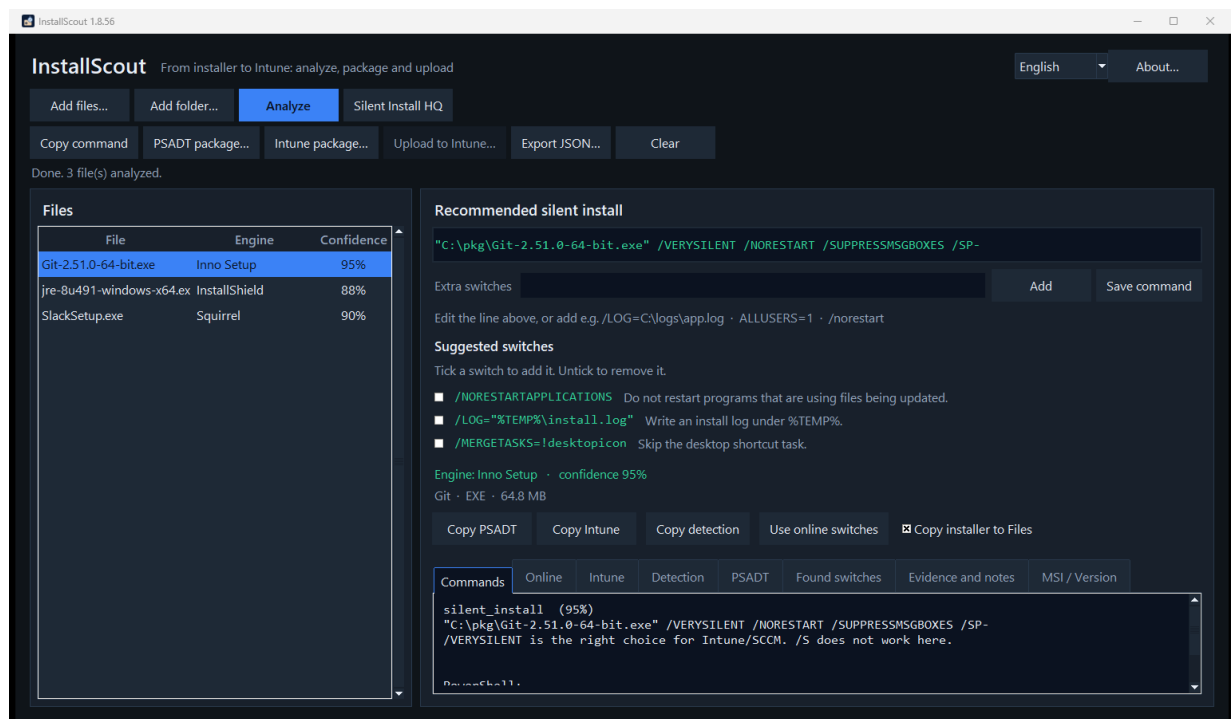
Figure 2. Git analyzed as Inno Setup with VERYSILENT.
