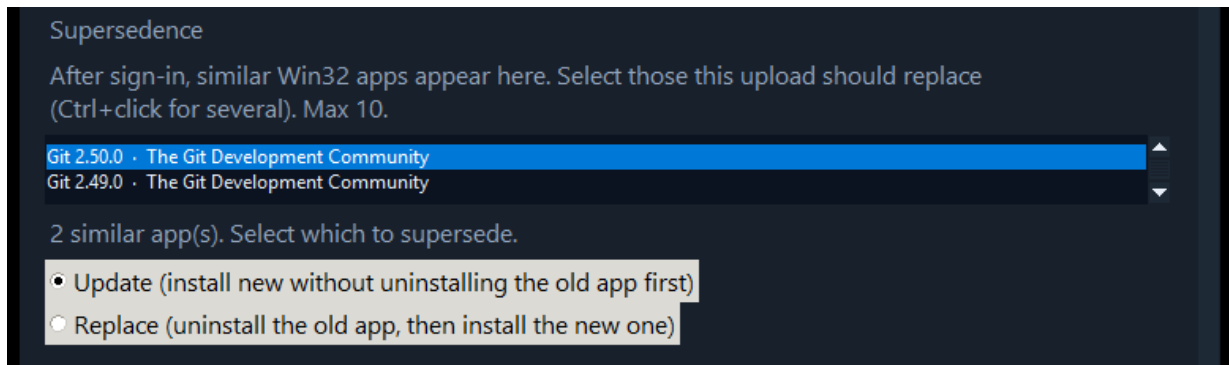
Figure 10. Supersedence in Upload to Intune: Git 2.50.0 selected, Update is the default.
