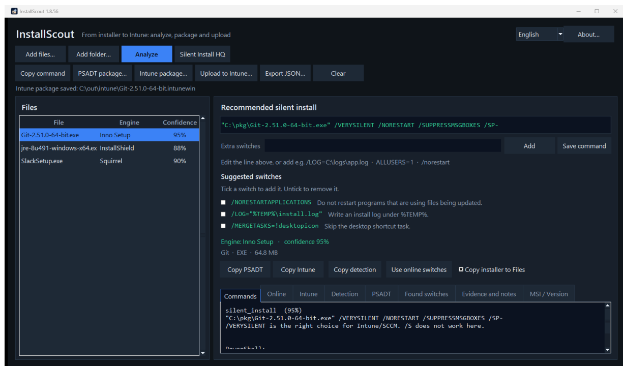
Figure 8. Upload to Intune is active when a local .intunewin exists.
