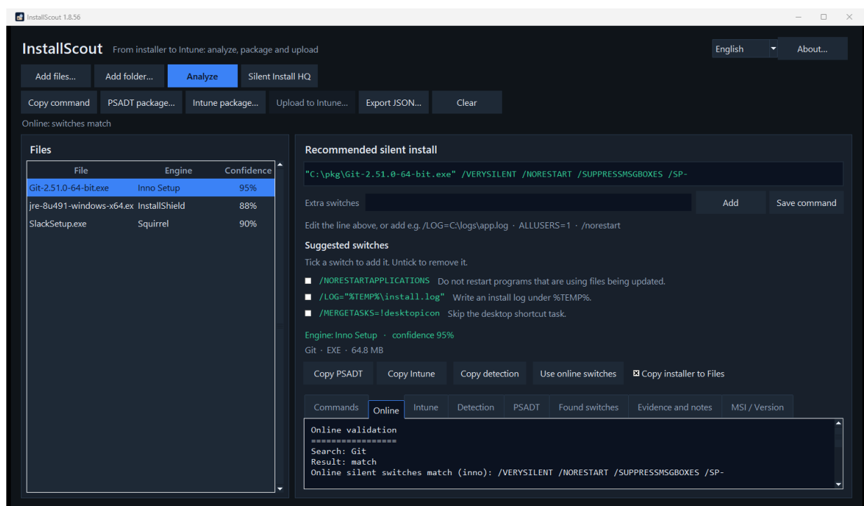
Figure 5. Online match for Git.
