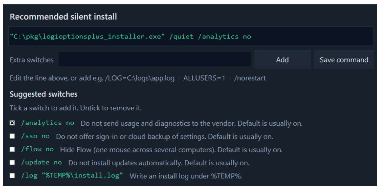
Figure 4. Suggested switches. Tick a box to add the switch. Here /analytics no is selected.
