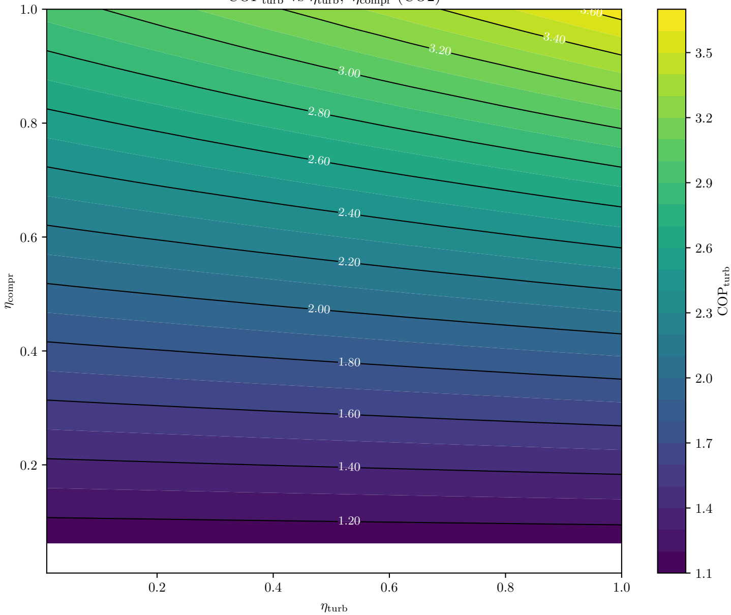
COP turb vs \eta_{\text{turb}} , \eta_{\text{compr}} (CO2)
