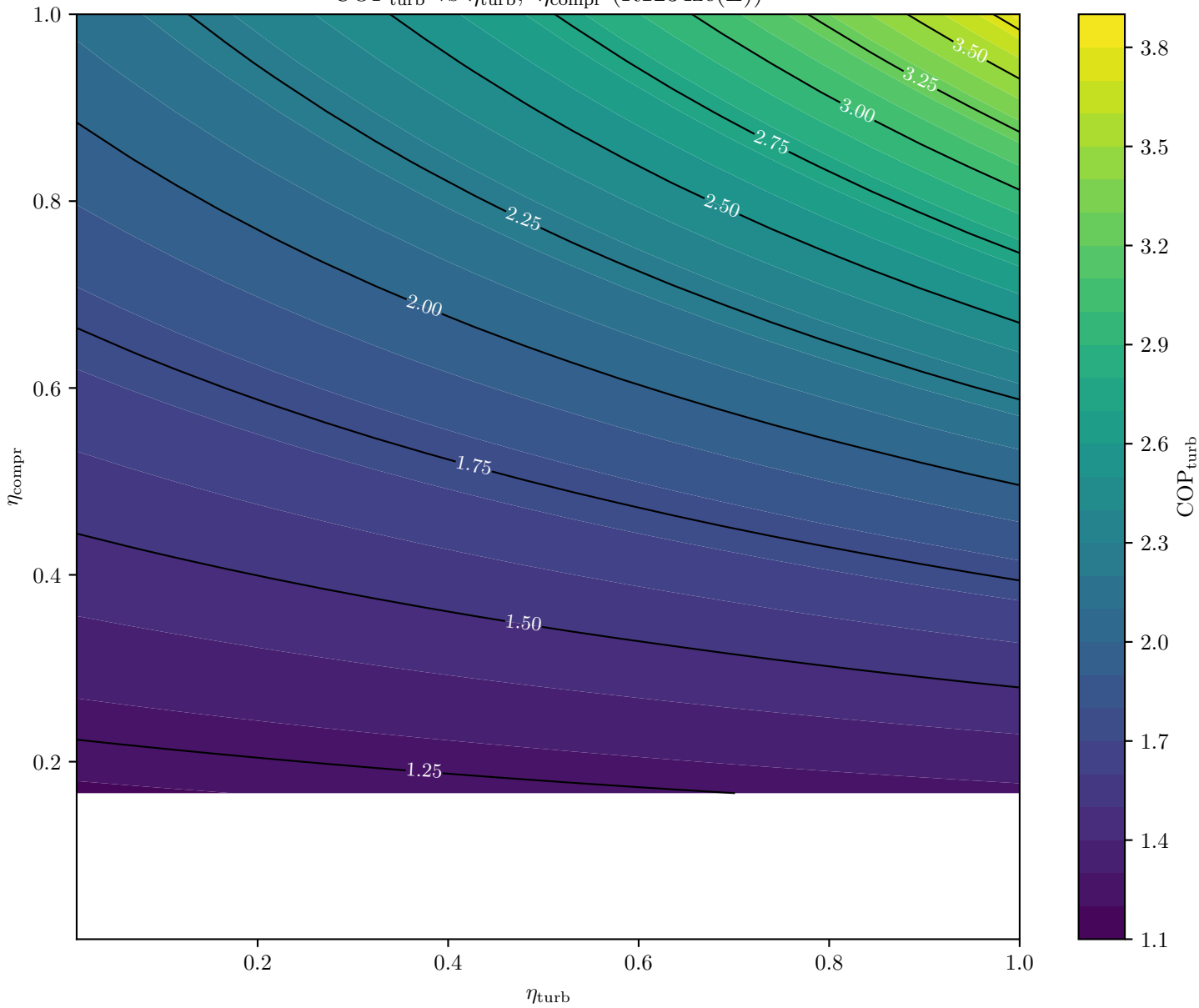
COP turb vs \eta_{\text{turb}} , \eta_{\text{compr}} (R1234ze(E))
