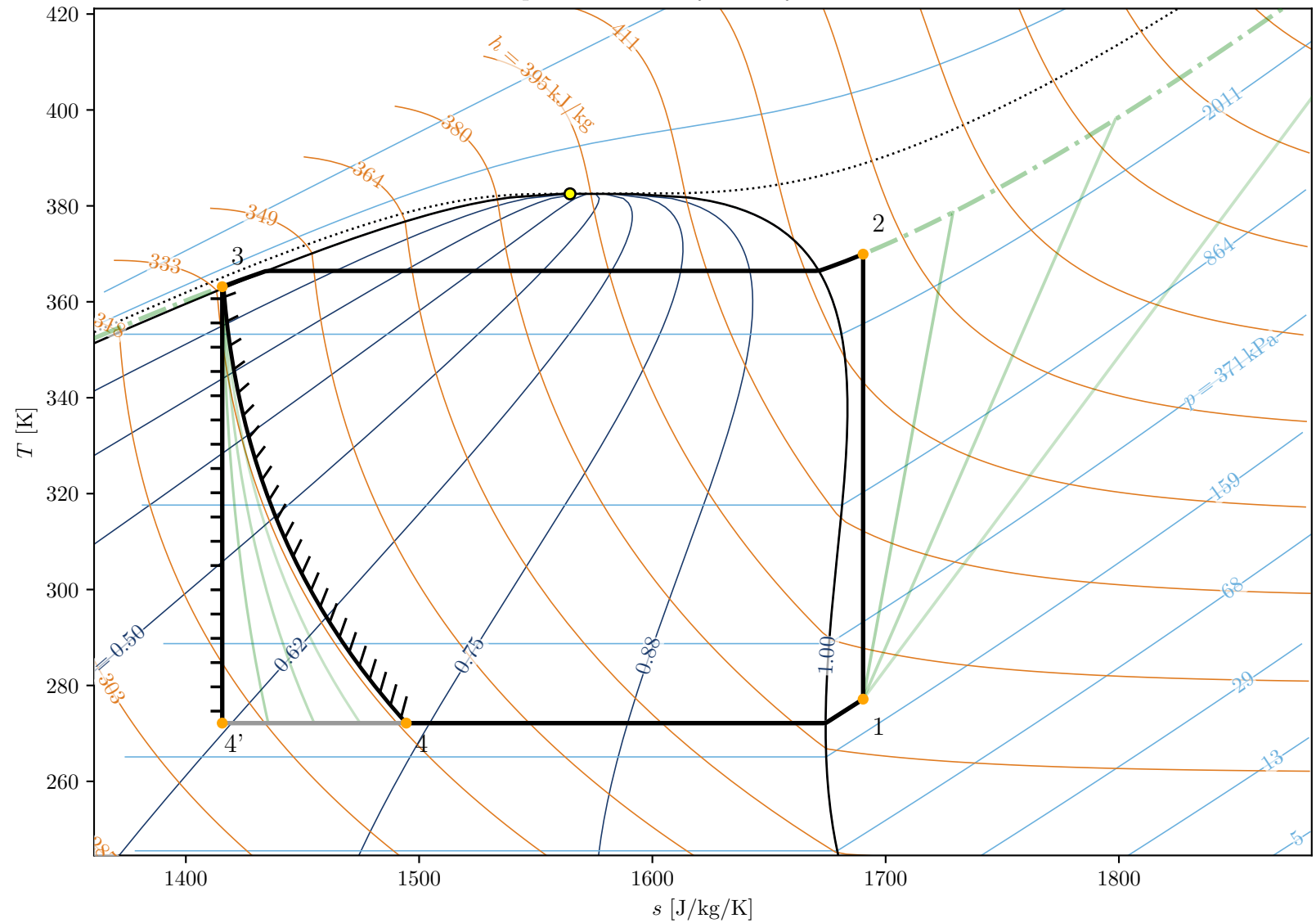
Compressor efficiency overlay at fixed PR
