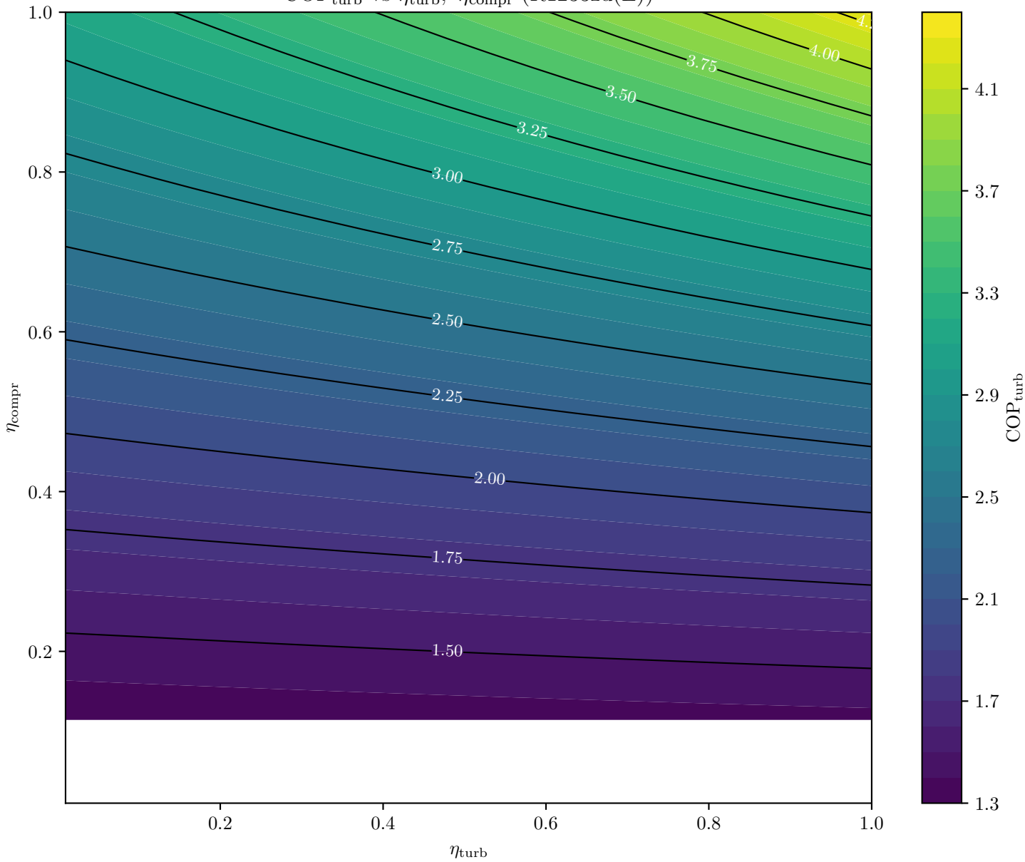
\text{COP}_{\text{turb}} vs \eta_{\text{turb}} , \eta_{\text{compr}} (R123zd(E))
