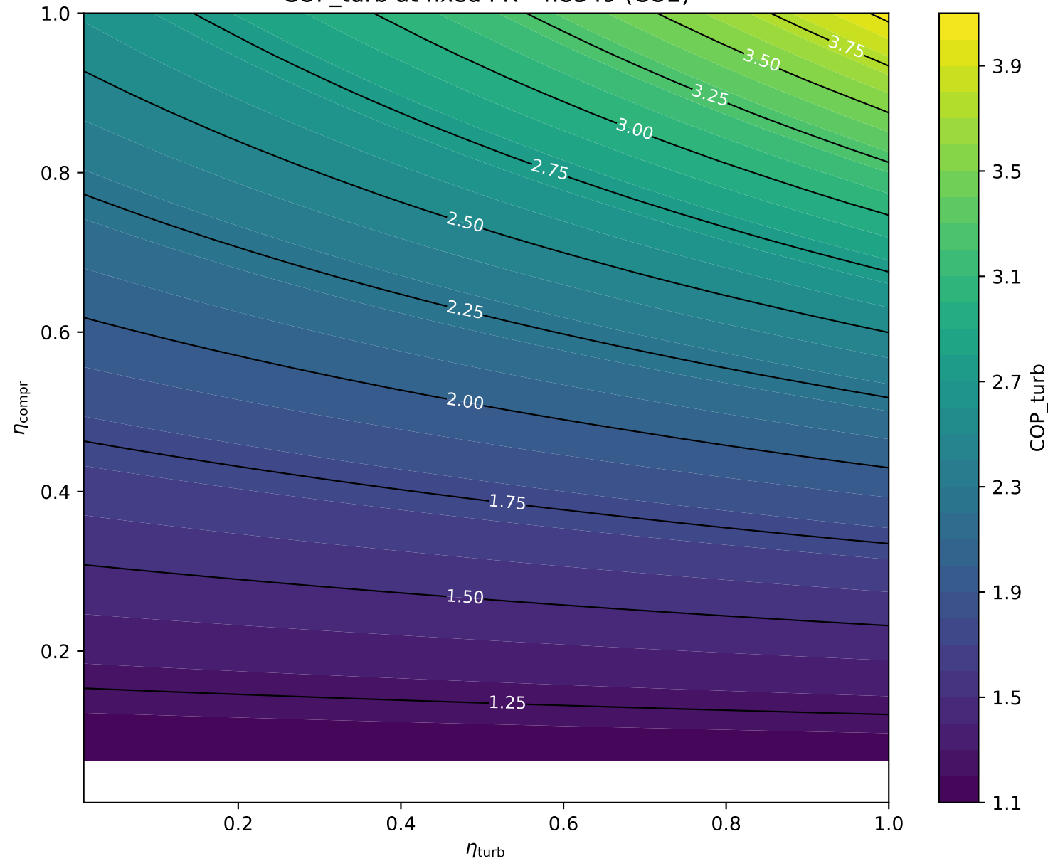
COP_turb at fixed PR=4.8349 (CO2)
