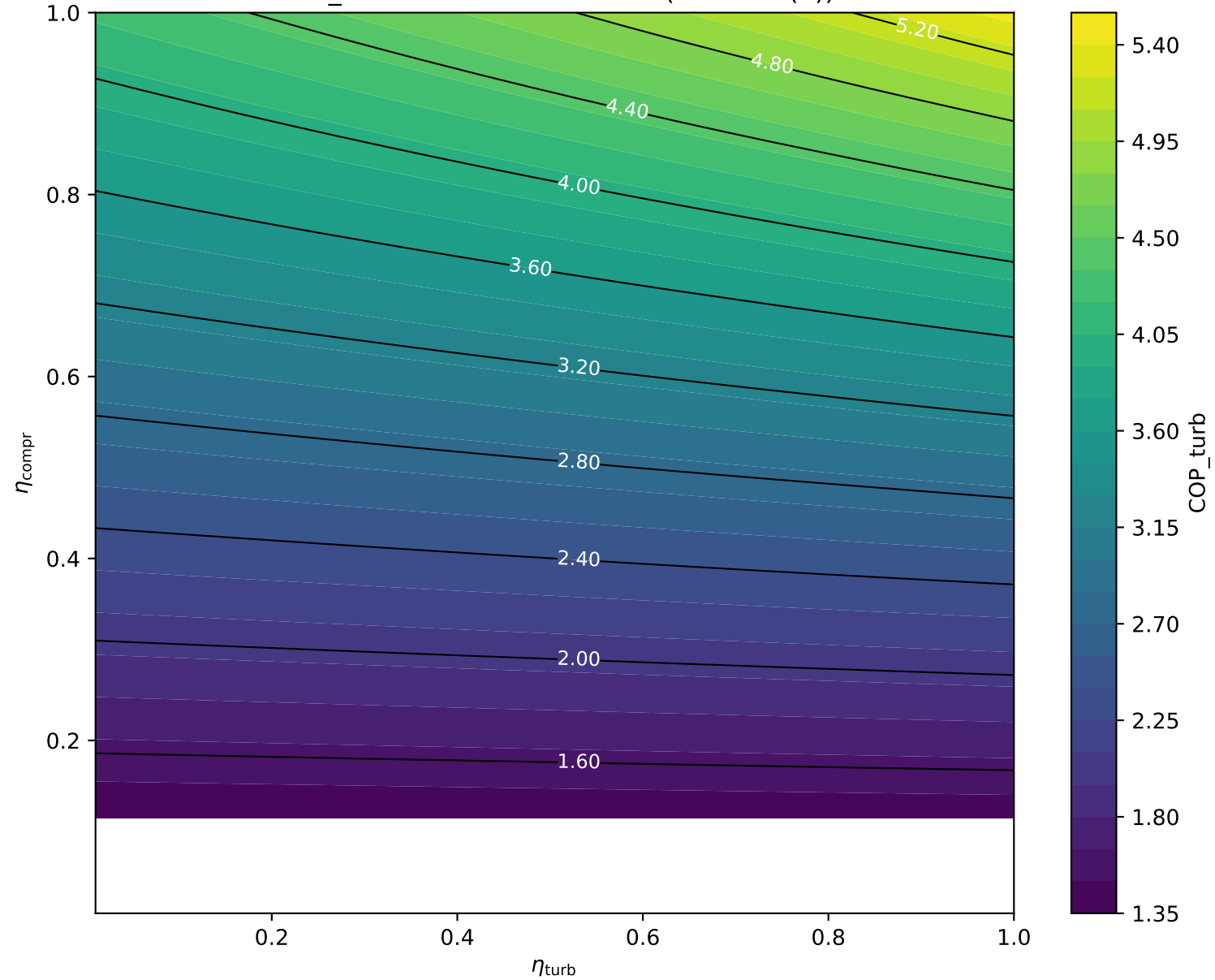
COP_turb at fixed PR=5.9604 (R1234ze(E))
