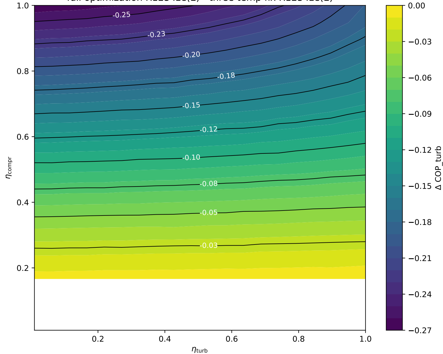
Absolute Deviation full optimization R1234ze(E) - three temp fix R1234ze(E)
