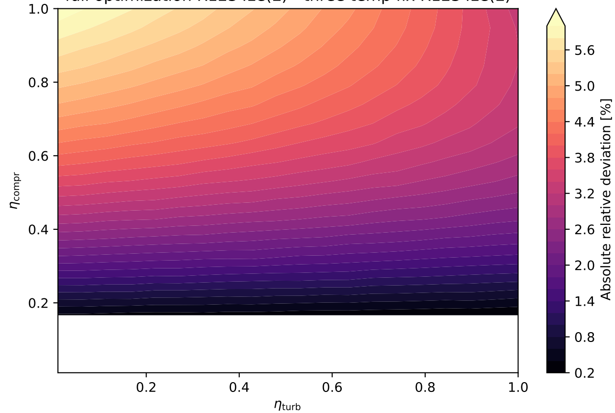
Relative Deviation full optimization R1234ze(E) - three temp fix R1234ze(E)
