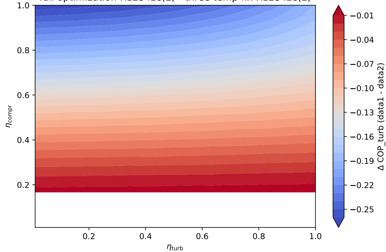
Absolute Deviation full optimization R1234ze(E) - three temp fix R1234ze(E)
