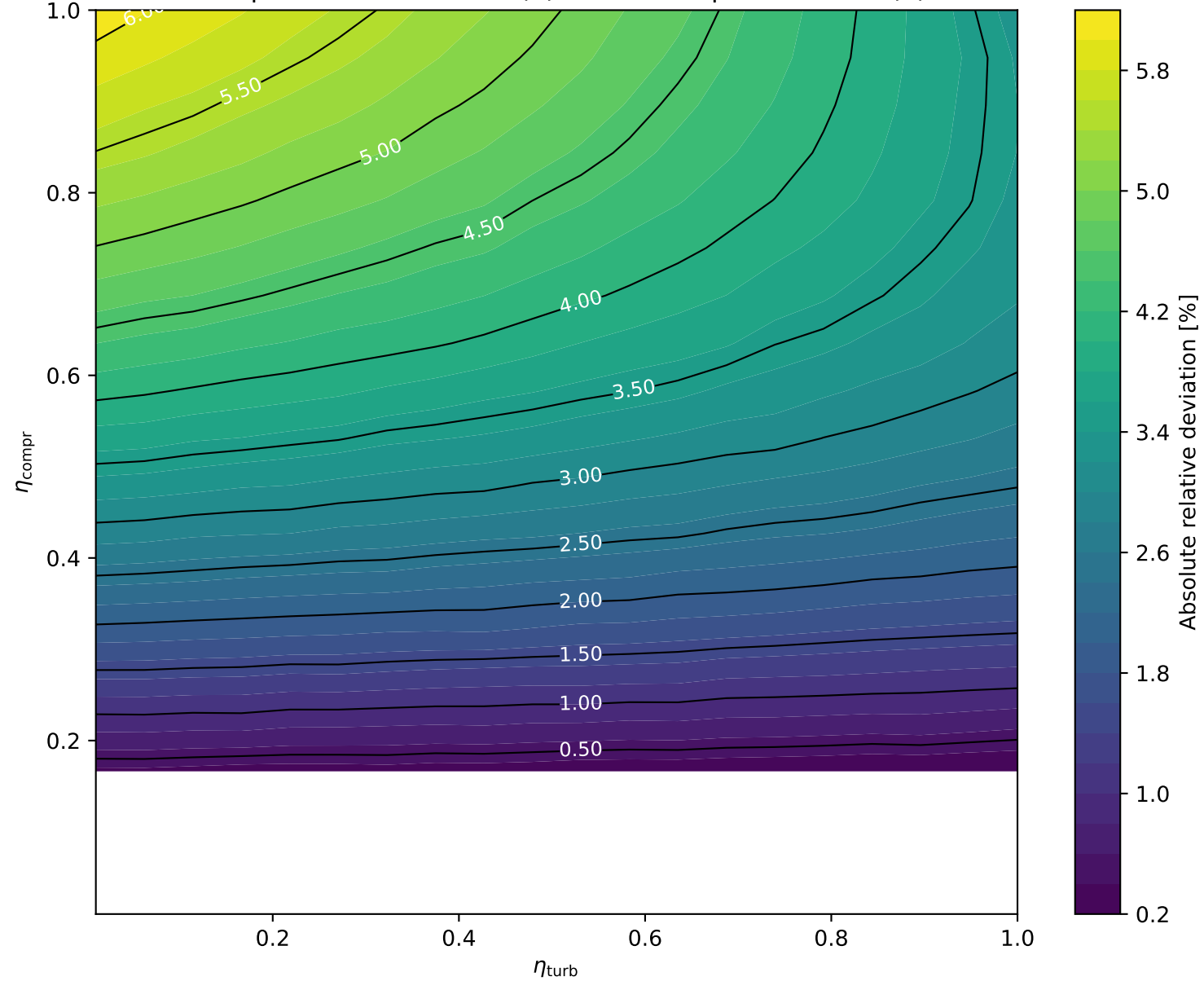
Relative Deviation full optimization R1234ze(E) - three temp fix R1234ze(E)
