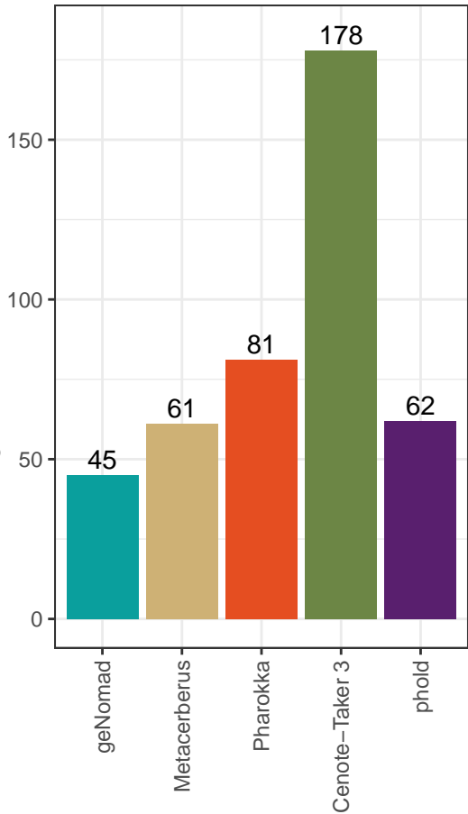
Single Copy MCP/TerL/Portal
