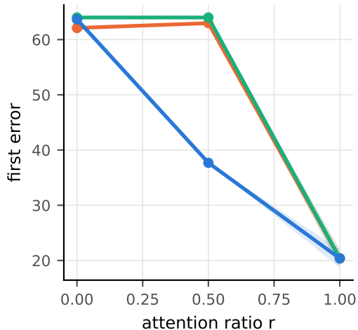
L=64, group=parity
