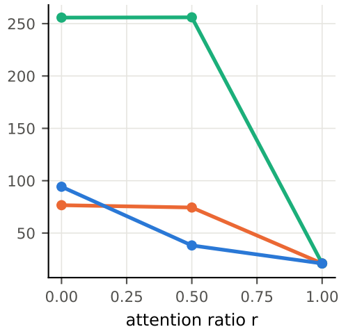
L=256, group=parity
