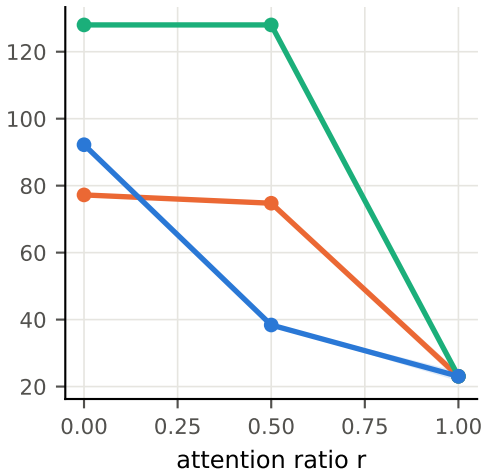
L=128, group=parity
