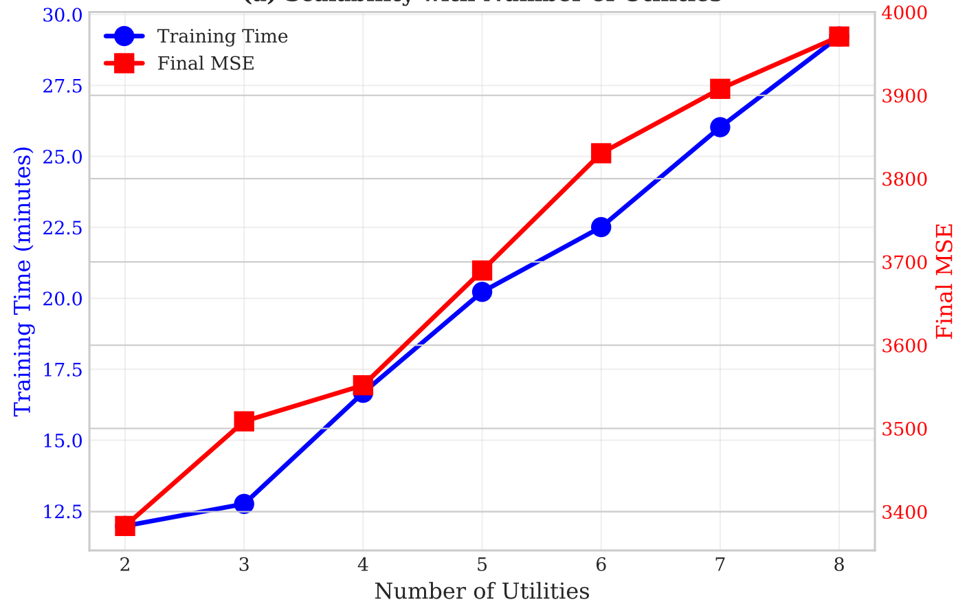
(a) Scalability with Number of Utilities
