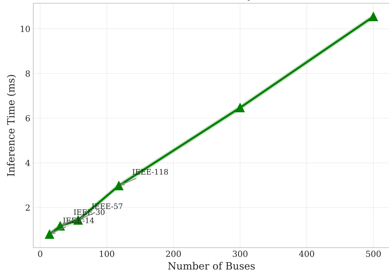
(b) Inference Time vs System Size
