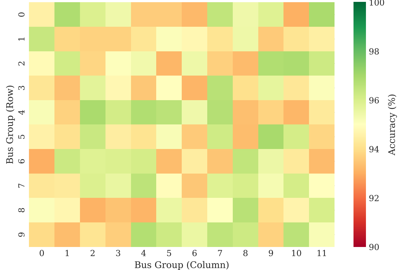
(a) Voltage Prediction Accuracy by Bus Region
