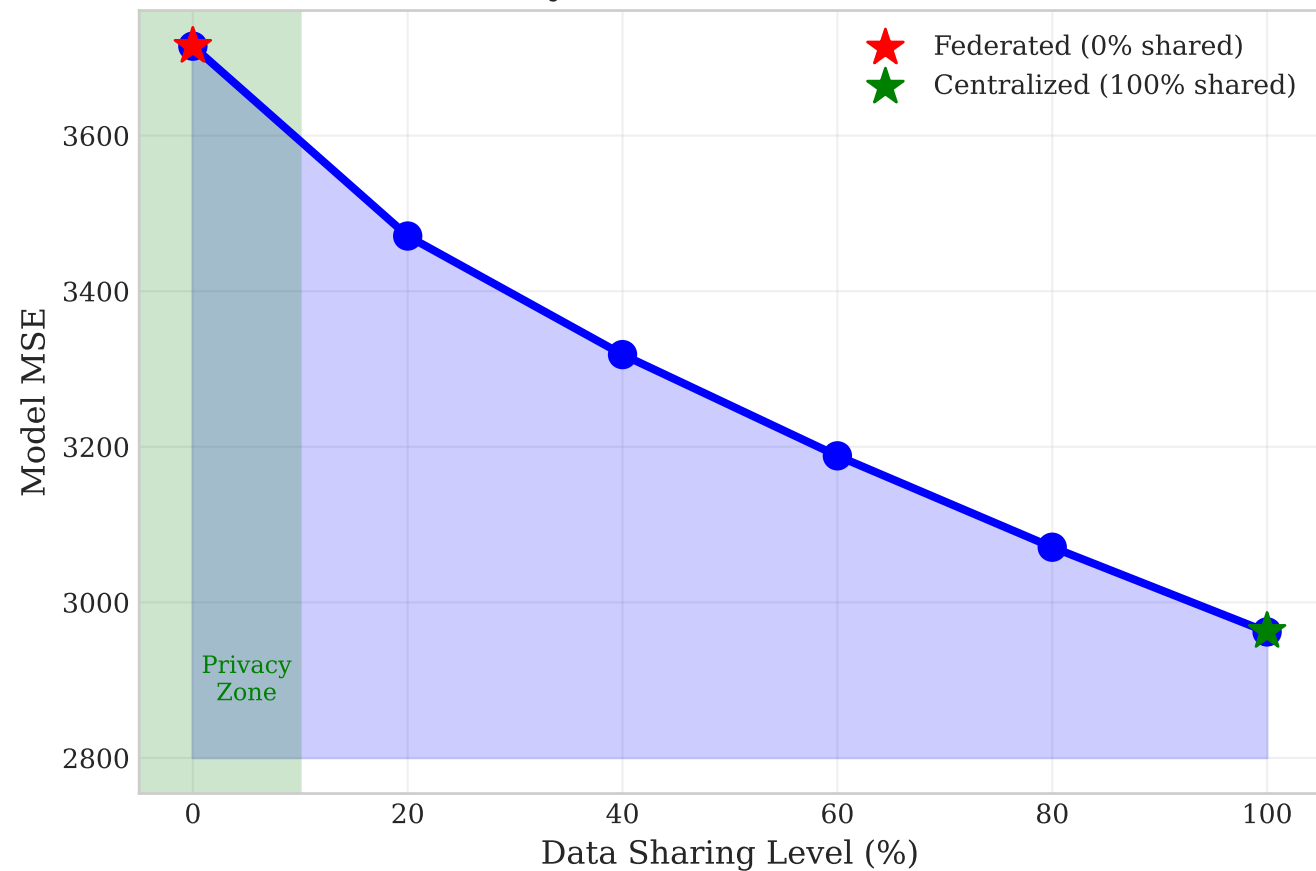
(b) Privacy-Performance Tradeoff Curve
