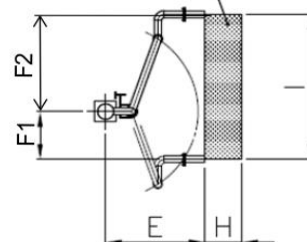
Connection vehicle side
