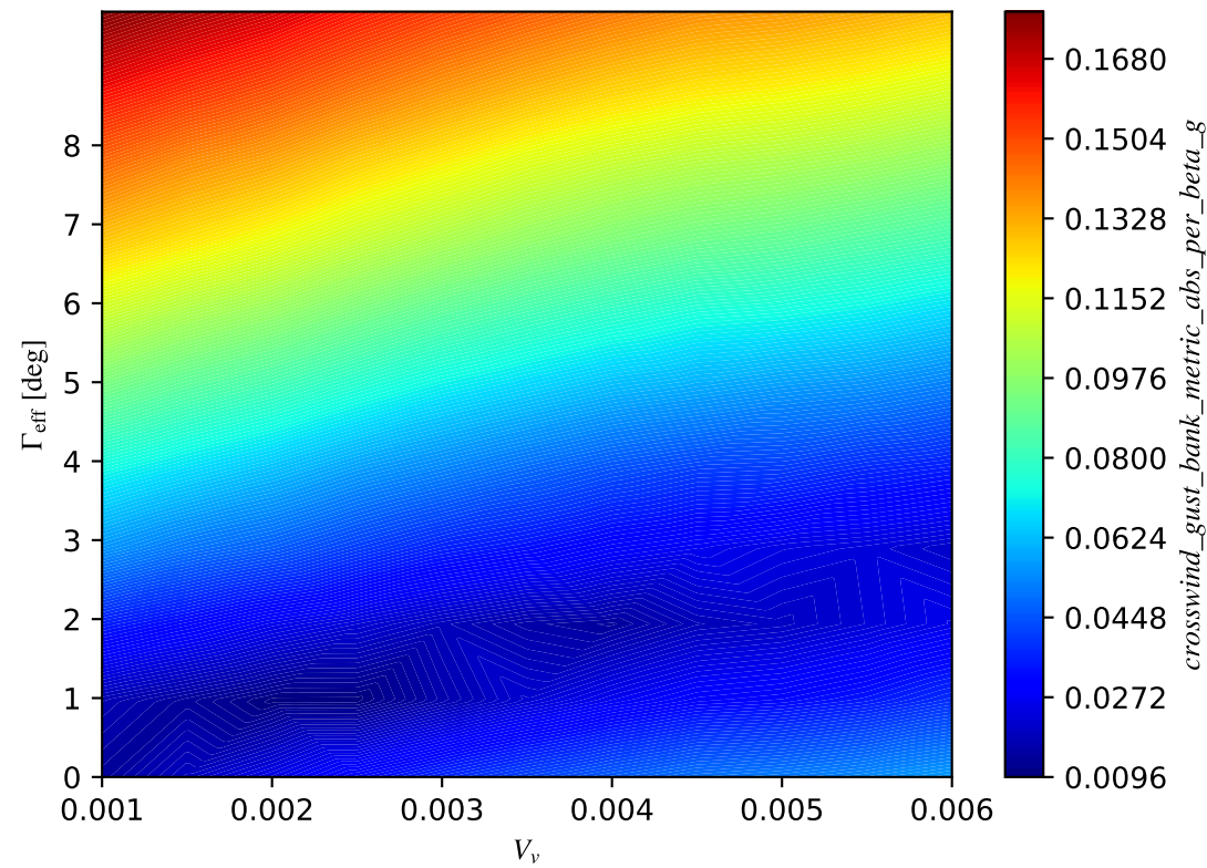
crosswind_gust_bank_metric_abs_per_beta_g
