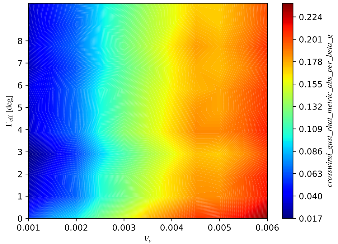
crosswind_gust_rhat_metric_abs_per_beta_g
