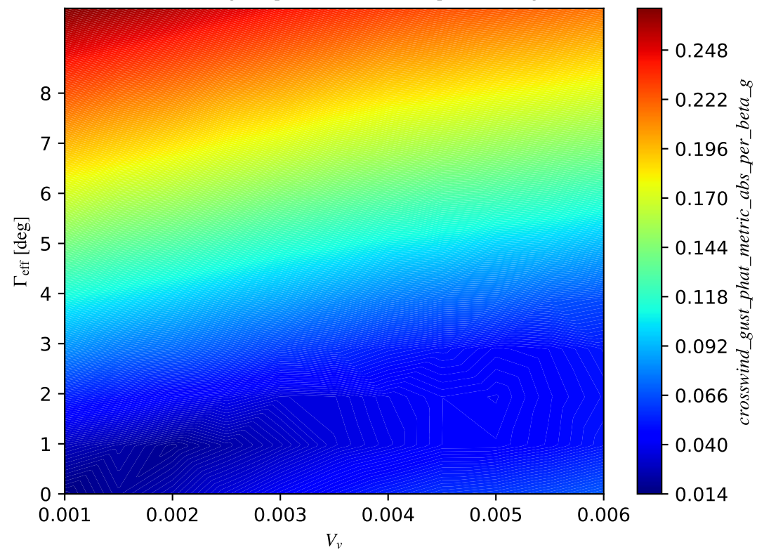
crosswind_gust_phat_metric_abs_per_beta_g
