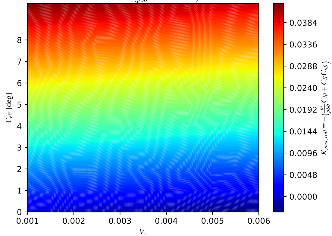
crosswind_gust_rhat_metric_abs_per_beta_g
