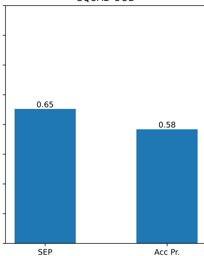
SQUAD OOD
