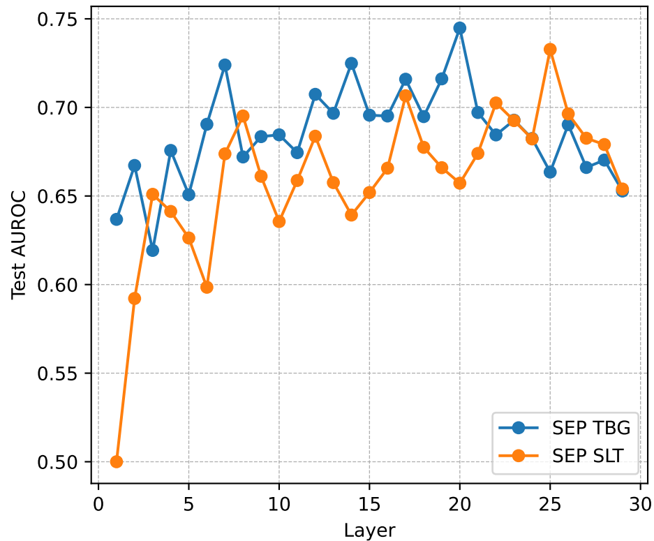
AUROC on SQUAD
