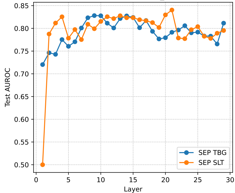
AUROC on TRIVIA_QA
