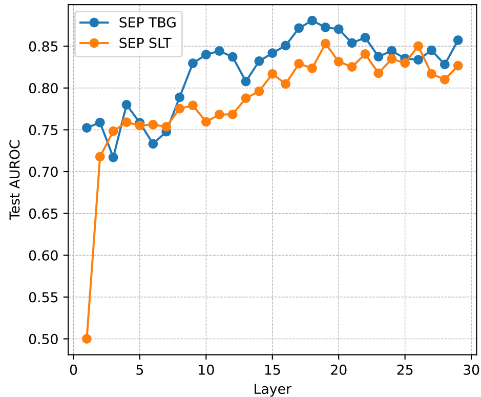
AUROC on NQ
