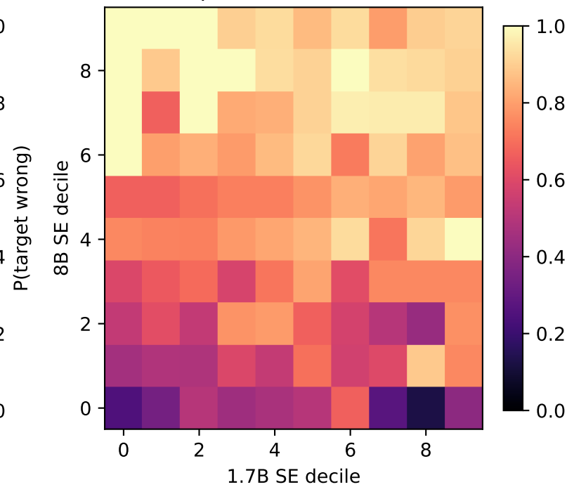
squad: 8B error rate
