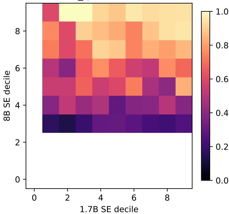
trivia_qa: 8B error rate
