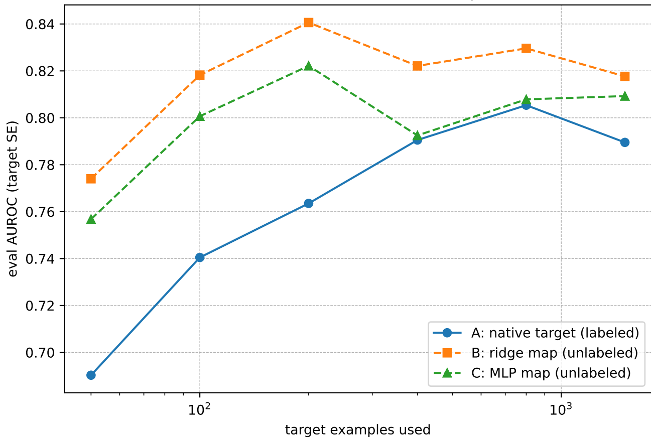
Linear vs nonlinear cross-scale map (SLT)
