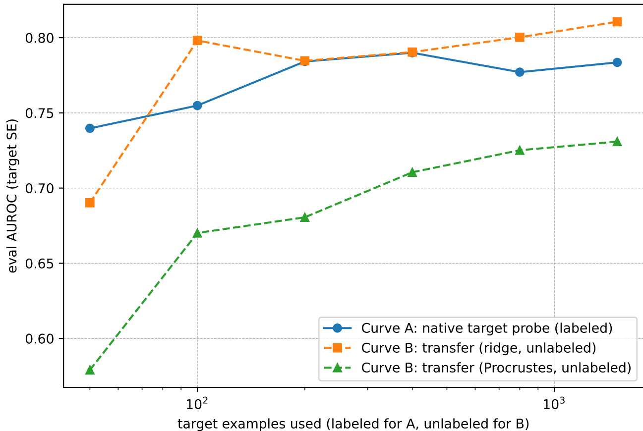
Cross-scale SE probe transfer (TBG, \alpha=1e+04 )
