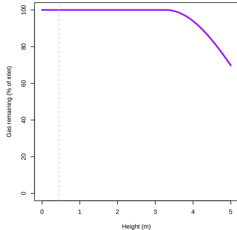
Gas-loss regime
