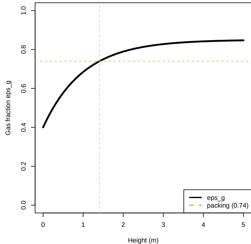
Holdup / interface
