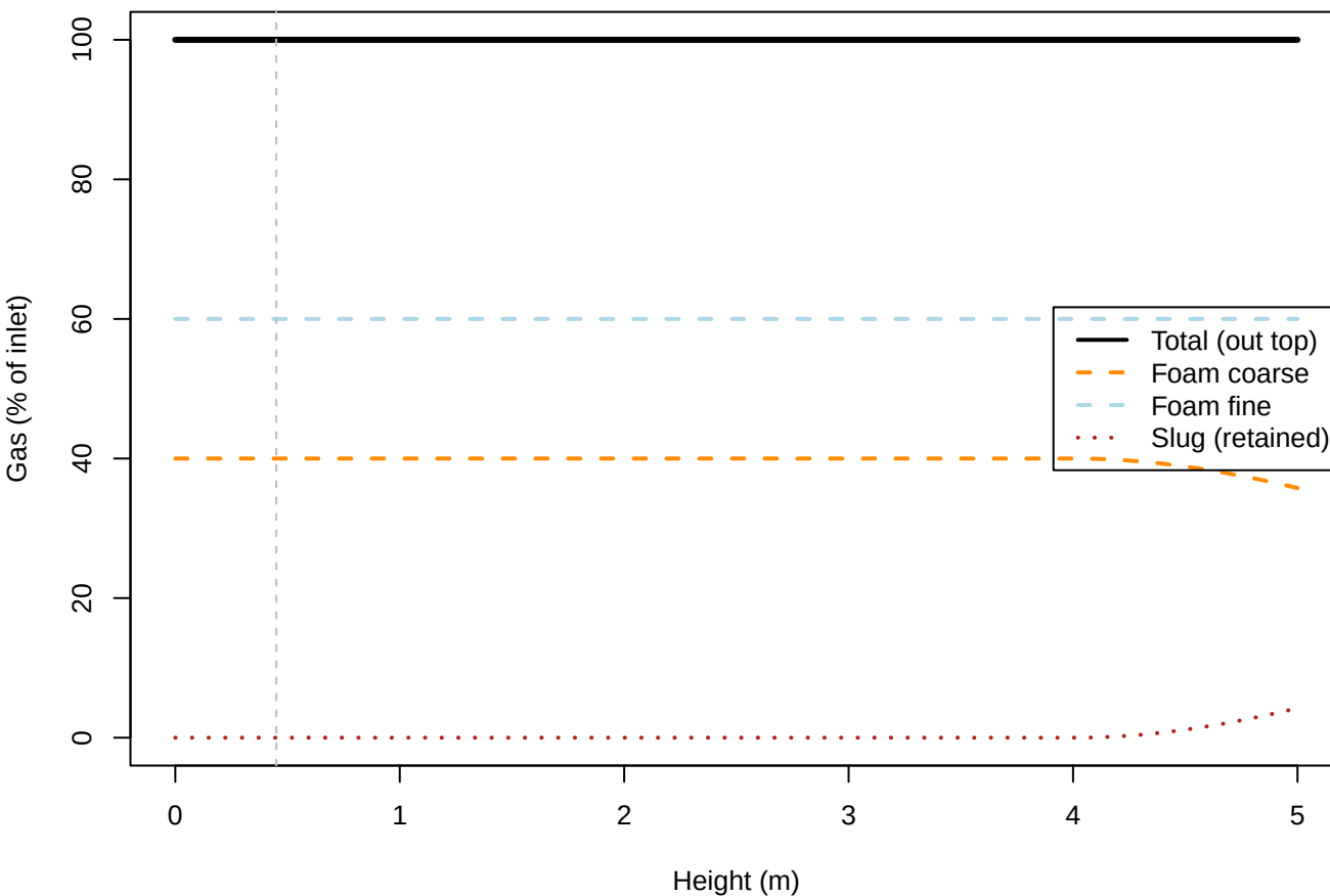
Gas state (conserved, bimodal foam)
