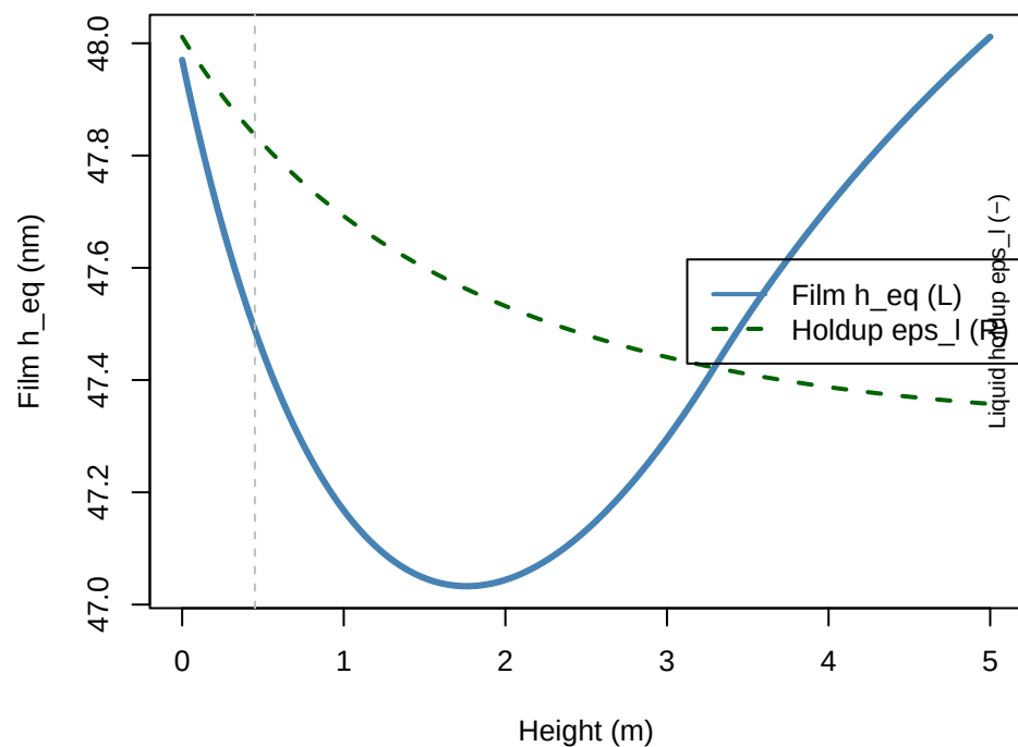
Film thickness & holdup
