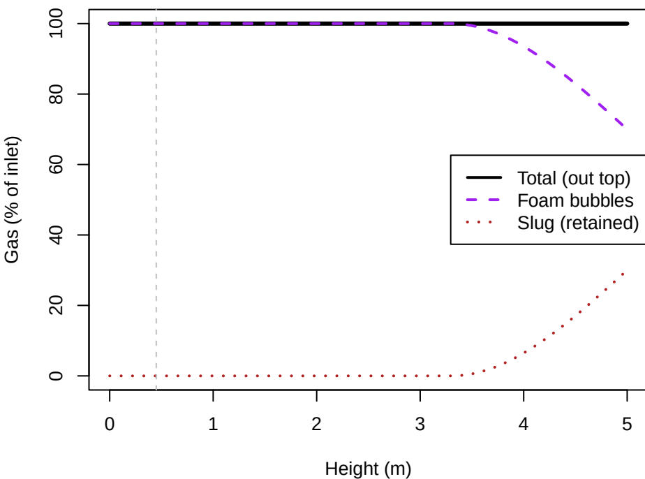
Gas state (conserved)
