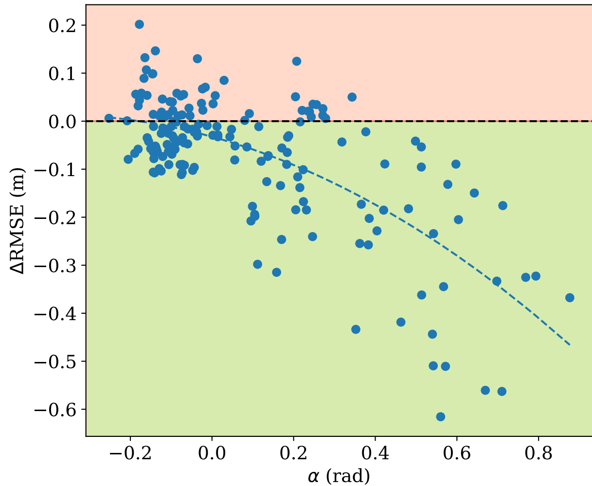
\Delta\text{RMSE} vs \alpha
