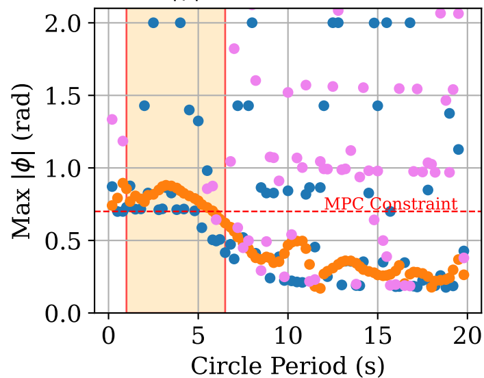
Max |\phi| x Circle Period (Zoom)
