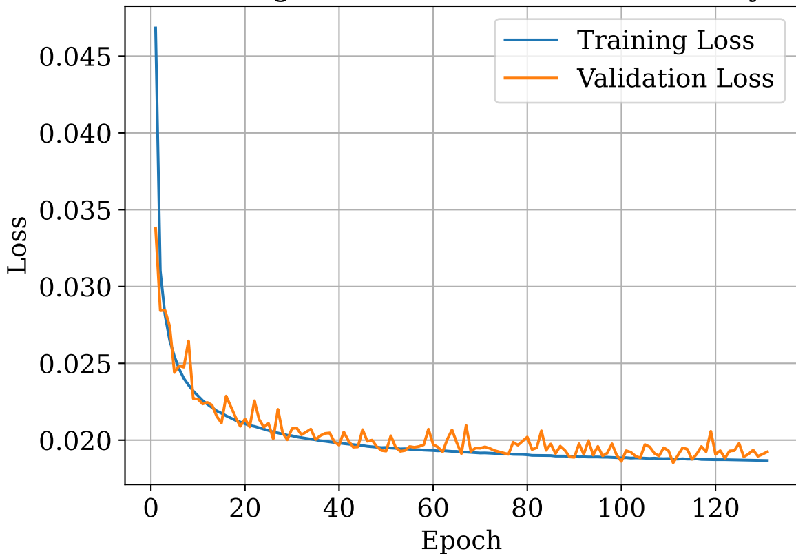
Training and Validation Losses History
