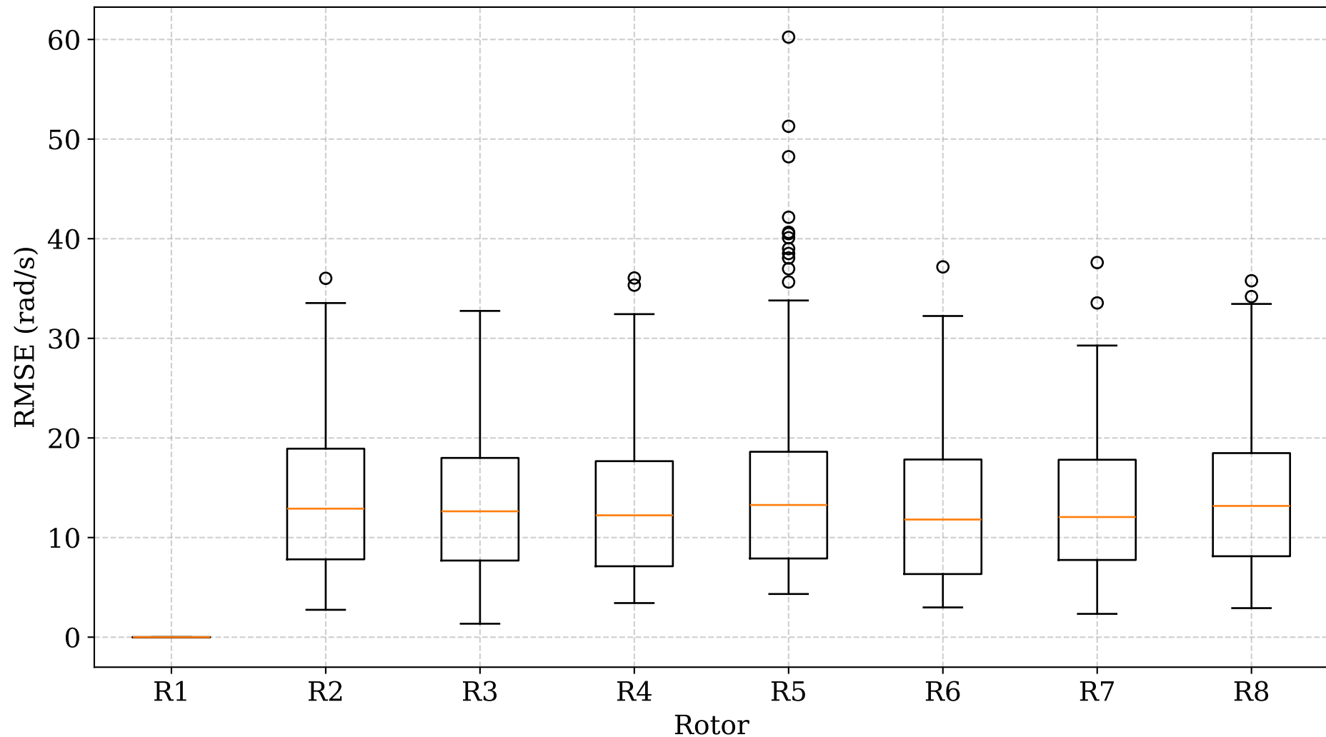
Rotor-wise RMSE Between NN and MPC Across Scenarios
