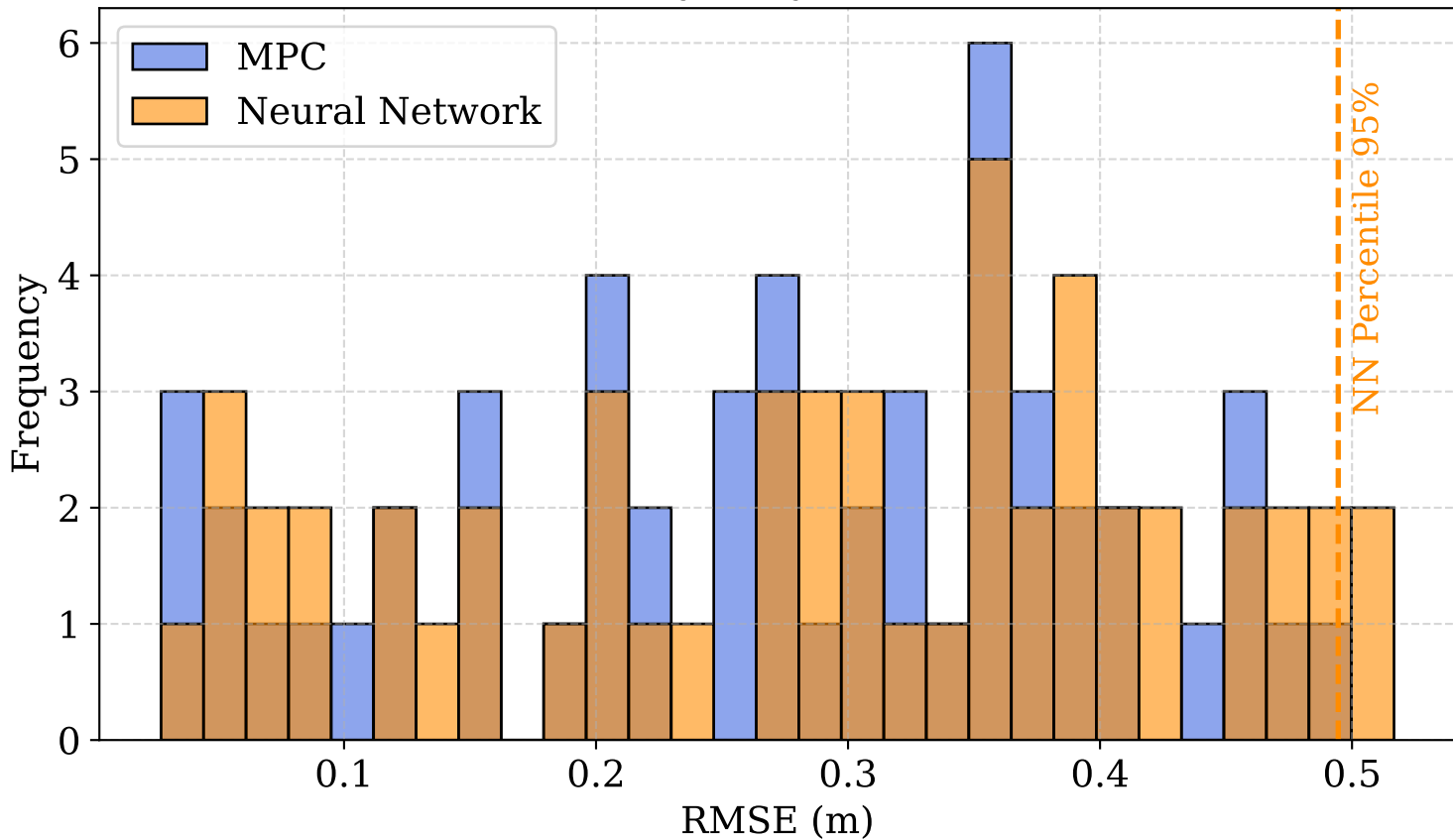
MPC and NN Trajectory RMSE Distributions
