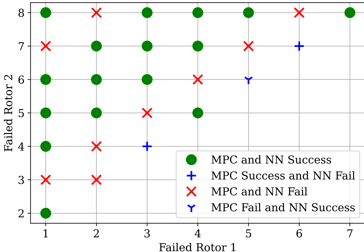
Successful and Failed MPC-NN Simulations with 2 Rotor Failures
