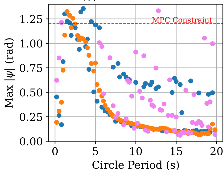
Max |\psi| x Circle Period (Zoom)
