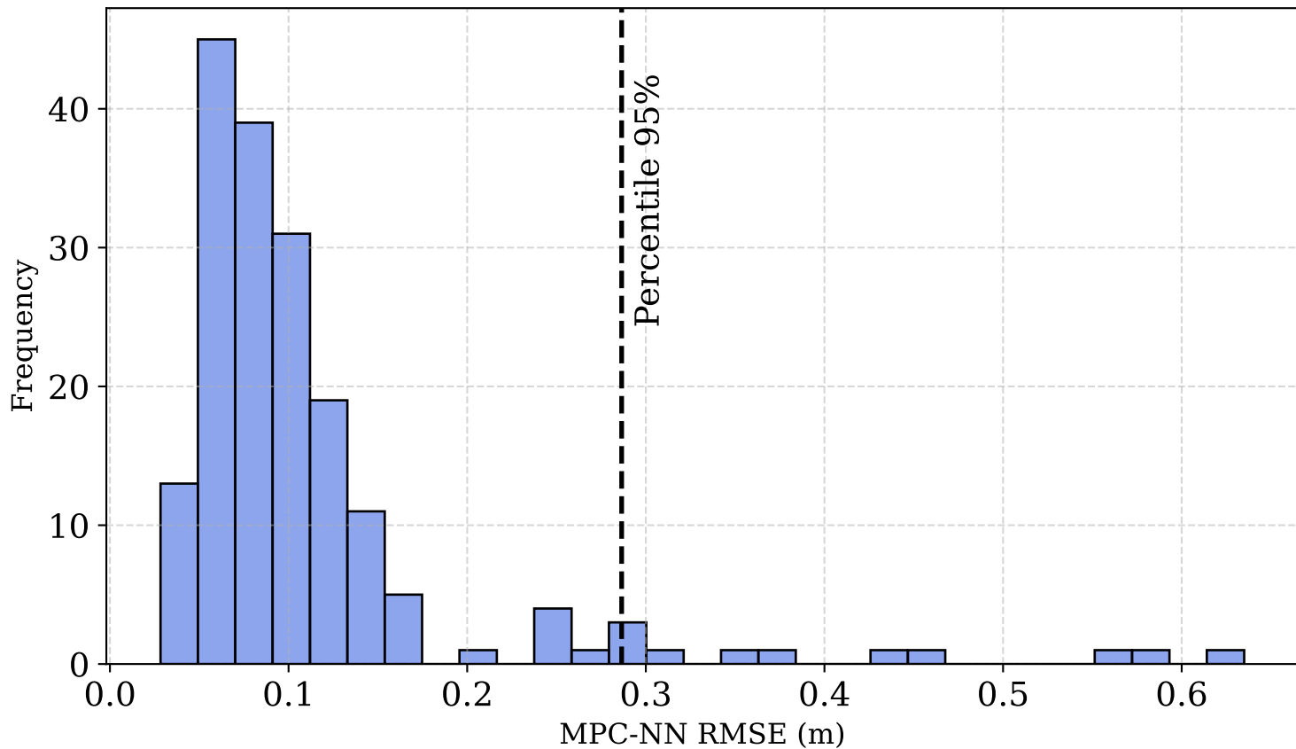
MPC-NN Position RMSE
