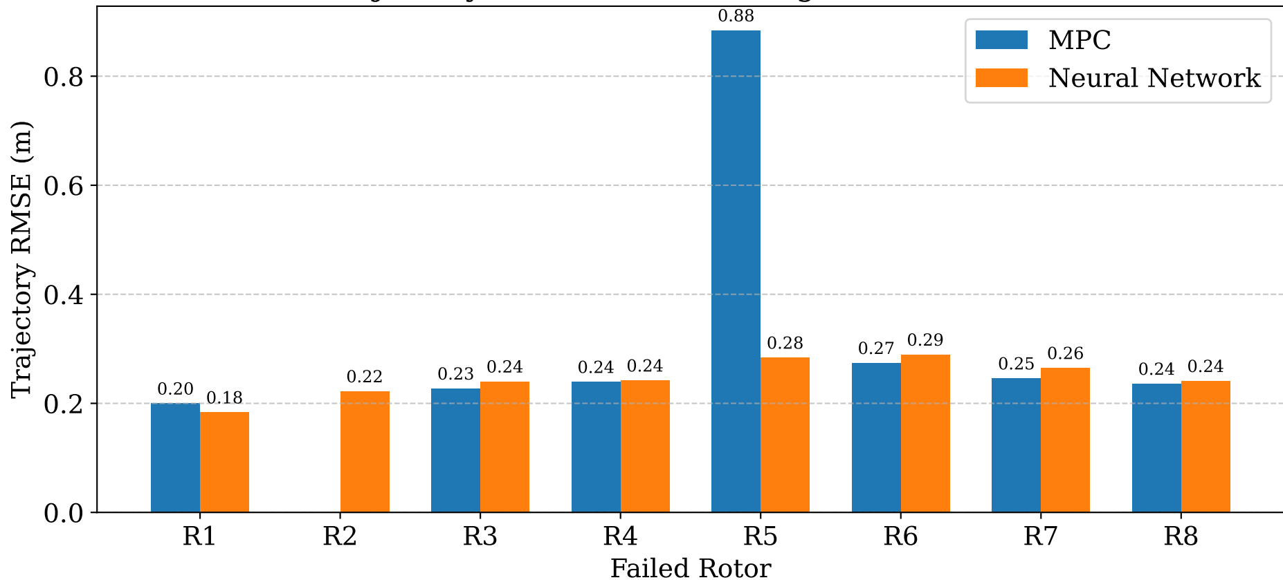
Trajectory RMSE for Each Single-Rotor Failure
