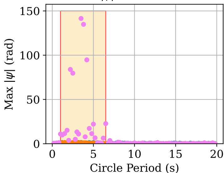
Max |\psi| x Circle Period
