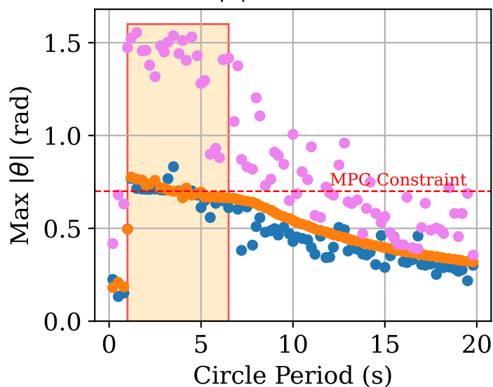
Max |\theta| x Circle Period
