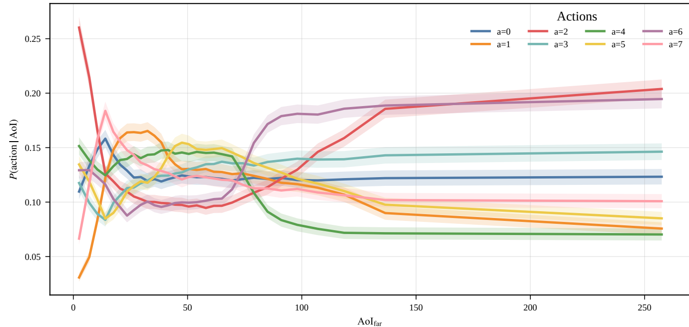
Policy Profiles vs AoI_{\text{far}}
