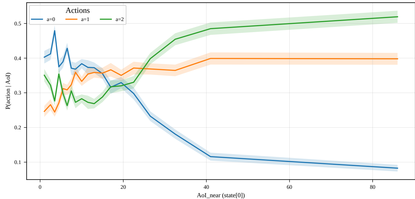
Policy Profiles vs AoI_near (state[0])
