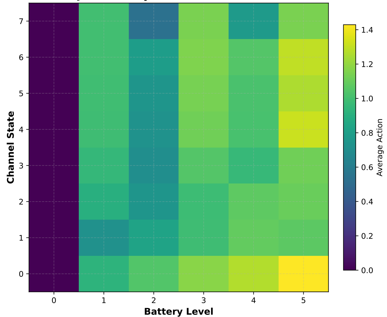
JAL: Battery vs Channel vs Action
