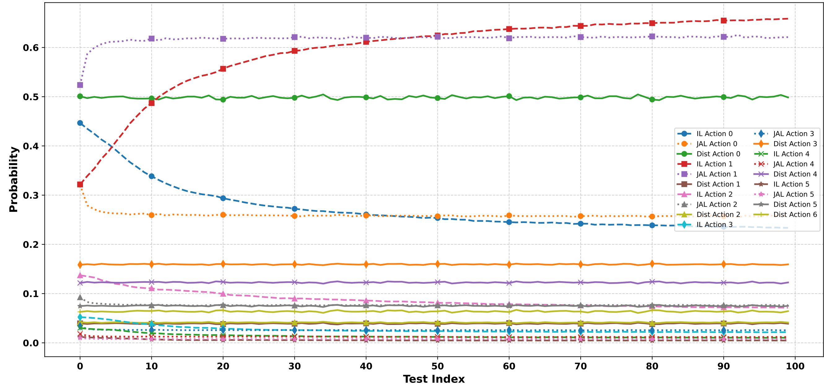
Action Probability Evolution Comparison G = 0.5
