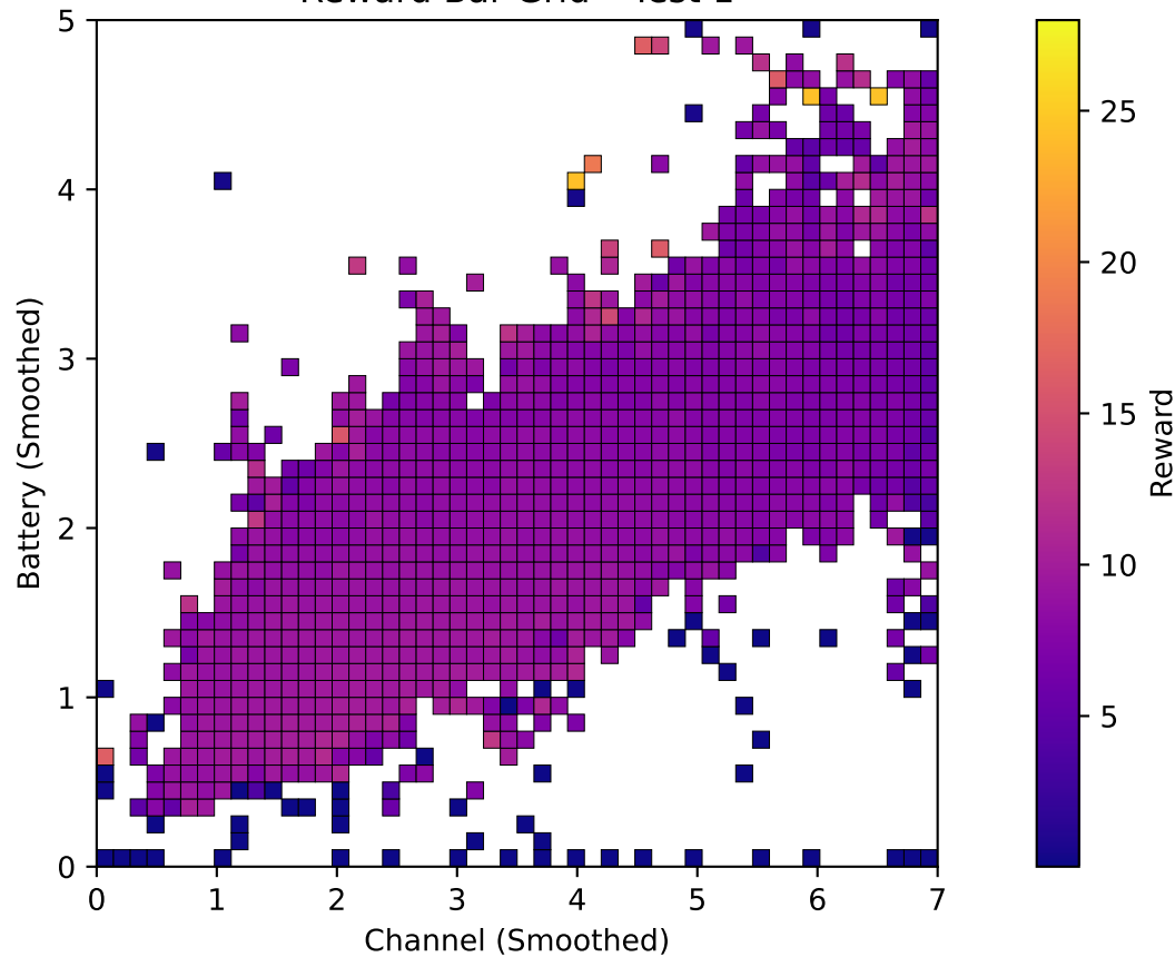
Reward Bar Grid - Test 1
