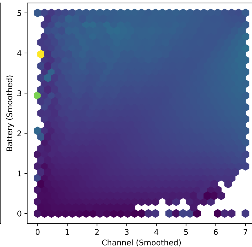
Action Hexbin - Test 2
