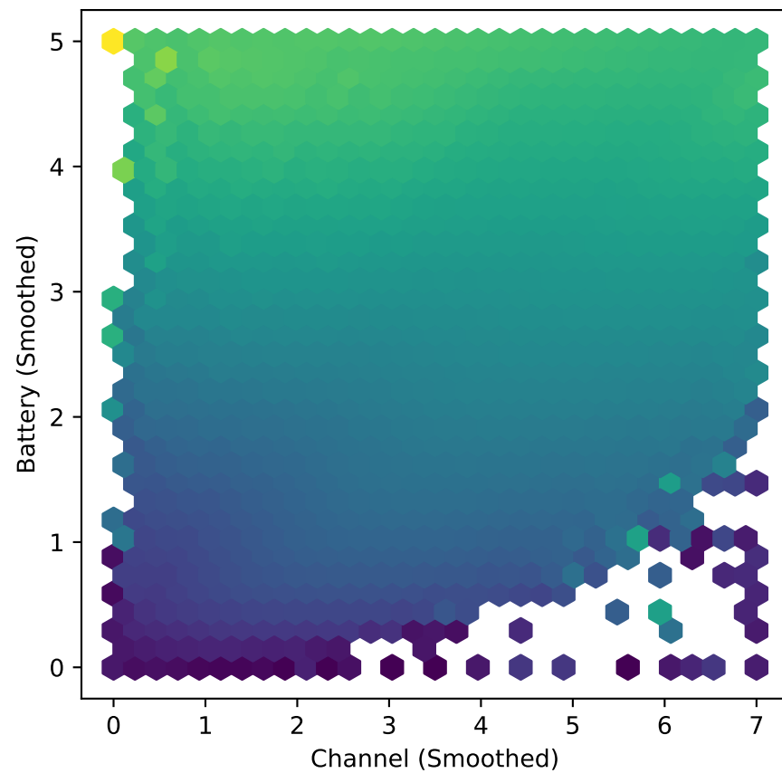
Reward Hexbin - Test 1
