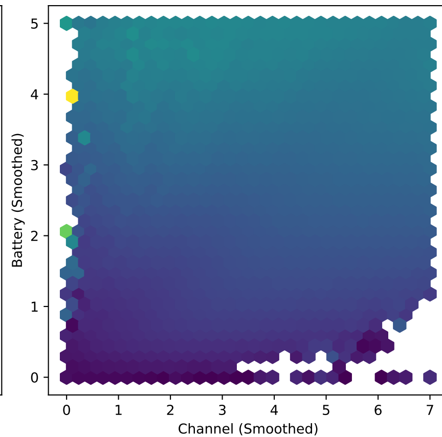
Reward Hexbin - Test 2
