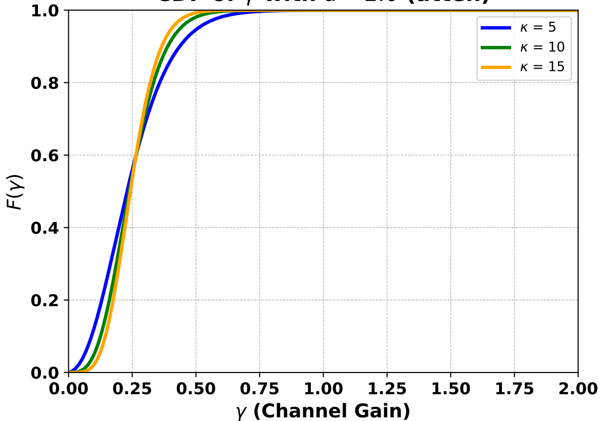
CDF of \gamma with d = 2.0 (atten)
