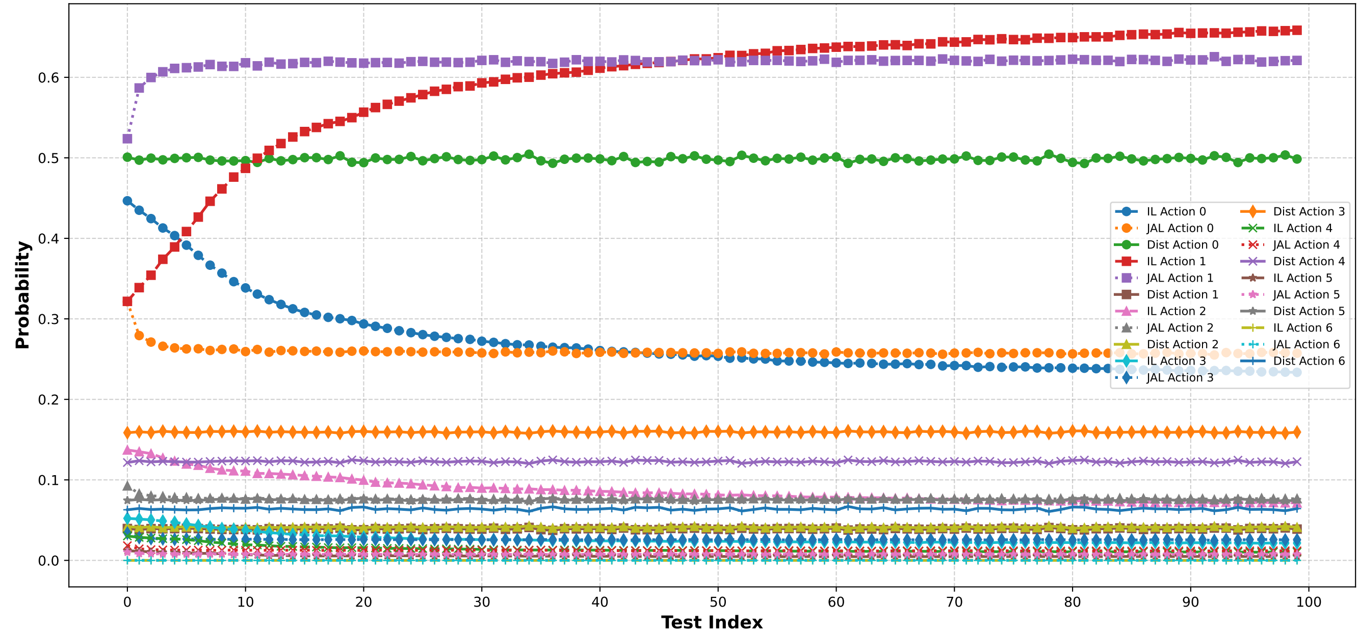
Action Probability Evolution Comparison G = 0.75
