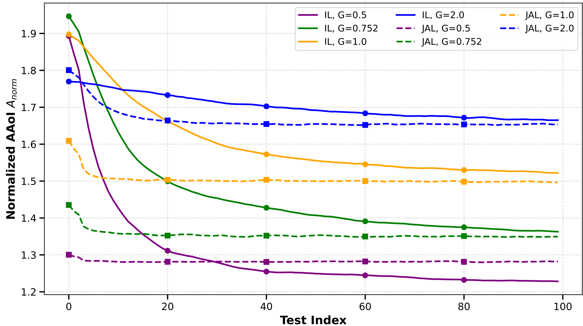
A_{norm} over Tests for IL and JAL at Various Gains
