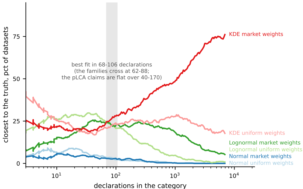
Which method is closest to the truth, by category size
