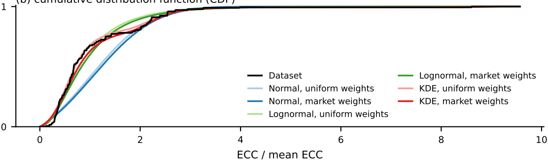
(b) cumulative distribution function (CDF)
